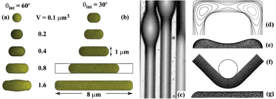
Figure 1 (a,b) Simulation results of sessile droplets of volume V = 0.1\text{--}1.6 \mu\text{m}^3 on a rectangular microstripe of dimensions 1 \mu\text{m} \times 8 \mu\text{m} . Exterior contact angle \theta_{\text{ext}} = 180^\circ ; interior contact angle (a) \theta_{\text{int}} = 60^\circ and (b) 30^\circ (Darhuber et al. 2000a). (c) Ribbons of water condensed from the vapor phase on hydrophilic microstripes about 50 \mu\text{m} in width. Above a critical volume such that \theta_B > 90^\circ , a bifurcation from uniform cross-section to a single bulge occurs, unlike a Rayleigh instability. [Reprinted with permission from Gau et al. (1999). Copyright AAAS.] (d,e) Top (contour) and side views of a liquid ribbon on a half loop pattern measuring 10 \mu\text{m} in length with \theta_{\text{int}} = 45^\circ and \theta_{\text{ext}} = 135^\circ . Liquid accumulates near the corners (Darhuber et al. 2000a). (f,g) Top and side views of a 10 \mu\text{m} wide liquid ribbon on a rounded corner pattern with \theta_{\text{int}} = 0^\circ and \theta_{\text{ext}} = 180^\circ . When the inner radius of curvature (indicated by the circle) is made to equal the microstripe width, bulges are eliminated for moderate fill volumes, and the liquid height profile becomes uniform (Darhuber et al. 2000a).
