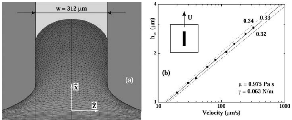
Figure 10 (a) Surface Evolver simulation of equilibrium capillary rise height for glycerol on a hydrophilic stripe ( \theta_{\text{int}} = 5^\circ and w = 312 \mu\text{m} ) patterned on a hydrophobic substrate ( \theta_{\text{ext}} = 95^\circ ) (Darhuber et al. 2000b). (b) Measurements of the entrained film thickness, h_\infty , versus the vertical withdrawal speed, U , on an isolated hydrophilic stripe (dimensions 49 \mu\text{m} \times 4 \text{mm} ) from a glycerol reservoir (Darhuber et al. 2000b).
