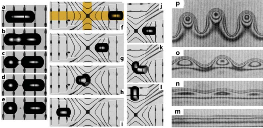
Figure 7 ( a–e ) Image sequence showing the thermocapillary splitting of a dodecane droplet on a partially wetting stripe ( w = 1000 \mu\text{m} , \Delta t_{\text{total}} = 8.5 \text{ s} ). The voltage applied to the embedded microheaters (electrical resistance 155 \Omega ) was 2.5 \text{ V} (Darhuber et al. 2003b). ( f–i ) Image sequence of dodecane droplet propelled by thermocapillary forces. Intersecting orange stripes designate partially wetting regions ( w = 1000 \mu\text{m} , \Delta t_{\text{total}} = 104 \text{ s} ) (Darhuber et al. 2003b). ( j–l ) Dodecane droplet turning a 90^\circ corner ( \Delta t_{\text{total}} = 164 \text{ s} ) (Darhuber et al. 2003b). ( m–p ) Evolution of fingering instability at the leading edge of a silicone oil film advancing on a chemically homogeneous substrate (silicon wafer) due to thermocapillary forces (applied shear stress \tau = 0.18 \text{ Pa} , \Delta t_{\text{total}} = 17 \text{ min} , instability wavelength \lambda \approx 500 \mu\text{m} ) (Cazabat et al. 1990).
