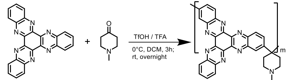
Figure 2. Schematic diagram of the synthesis of HATNA-based polymers
