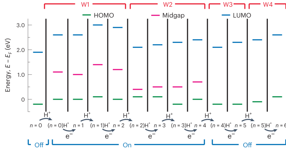
Figure 1. The mechanism of HATNA molecular switch
