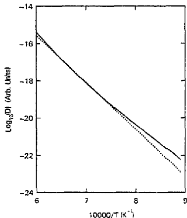
Fig. 1. Logarithmic plot of D_{\text{eff}} = D_1 \exp(-Q_1/kT) + D_2 \exp(-Q_2/kT) with Q_1 = 4 eV and Q_2 = 6 eV and D_2/D_1 = 5:1 (solid line), compared with a plot of D = D_0 \exp(-Q/kT) with Q = 5 eV (dashed line) demonstrating that two terms may appear as a single exponential in a given temperature range.
