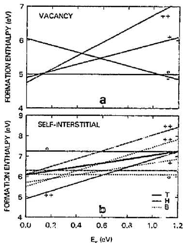
Fig. 3. Calculated formation enthalpies of various charge states \sigma : (a) the vacancy; and (b) the self-interstitial at three different sites (see fig. 4) in Si.
