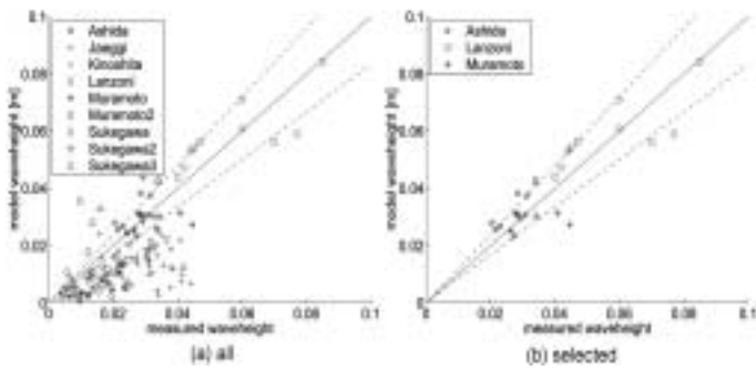
Fig. 6. The predicted wave height plotted against the measured values (a) for all experiments and (b) for the experiments with R\sqrt{Re} > 2000 . The dotted lines show the 20% error boundaries.
