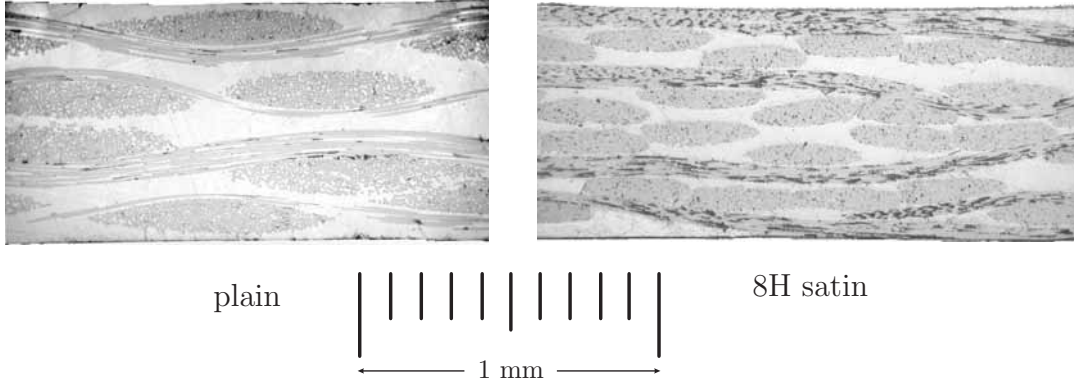
Figure 18: micrographs of the cross-section of a four layered orthogonal plain weave and 8H satin weave.
