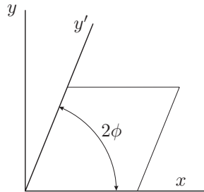
Figure 11: Shear transformation.
