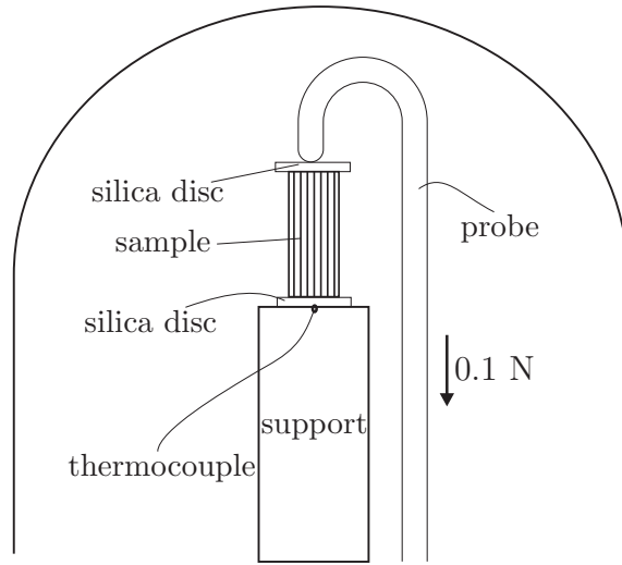
Figure 16: Set-up in TMA for measuring thermal expansion.
