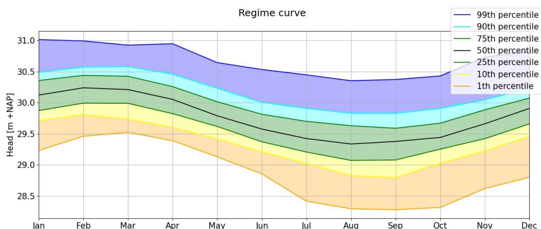
Figure 6: Example of a regime curve. The black line is the 50 th percentile, the median. The coloured lines could represent the p^{\text{th}} percentile, therefore the percentage of the groundwater levels that are below this line. The range between percentiles are classified to drought conditions.
