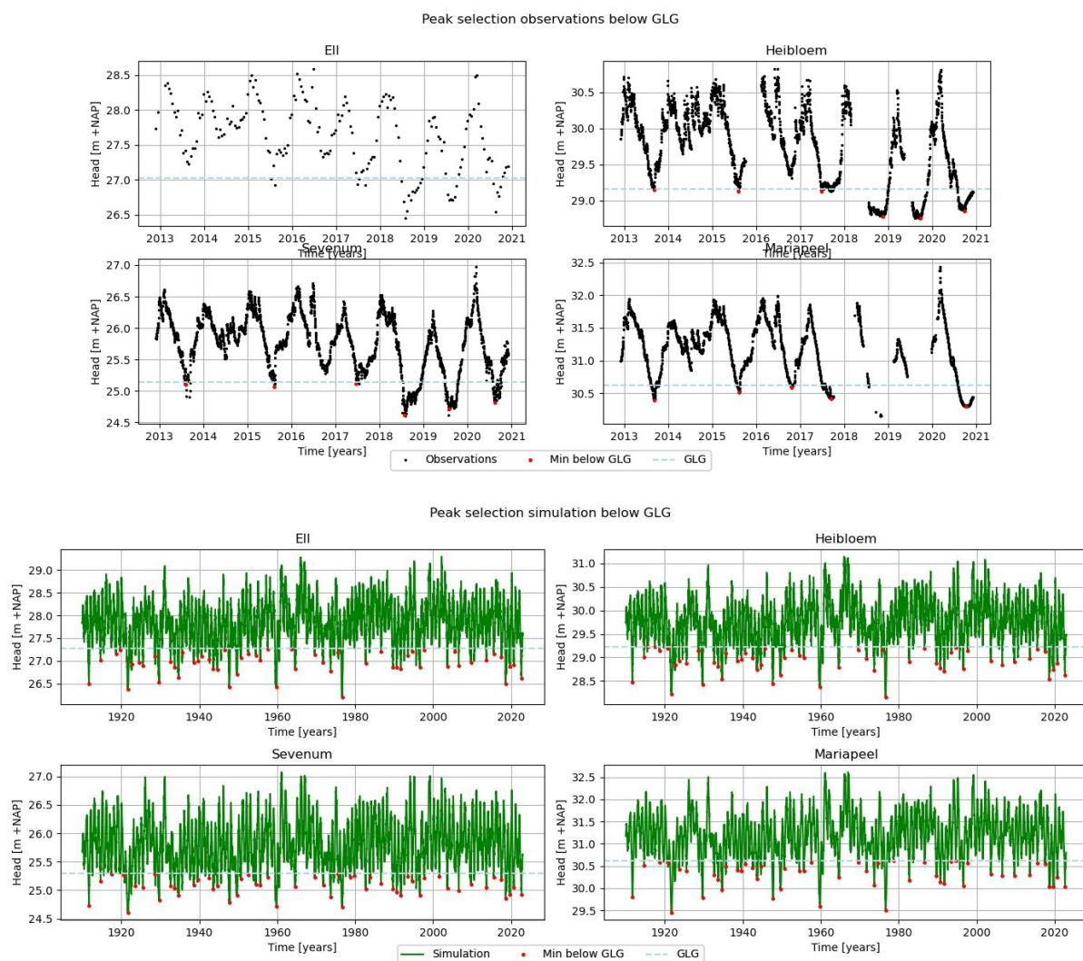
Figure 50: Selection of drought events with minimum groundwater head below GLG.
