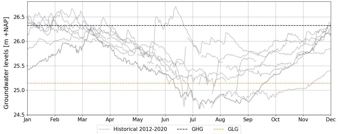
Figure 4: Describing the annual fluctuations of groundwater using the parameters GLG and GHG.
