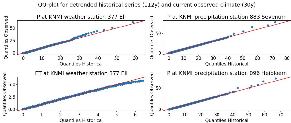
Figure 12: QQ-plots: quantiles of historical precipitation and reference crop evaporation are compared to quantiles of observed precipitation and reference crop evaporation. If the distributions are equal, the points will fall along a straight line.
