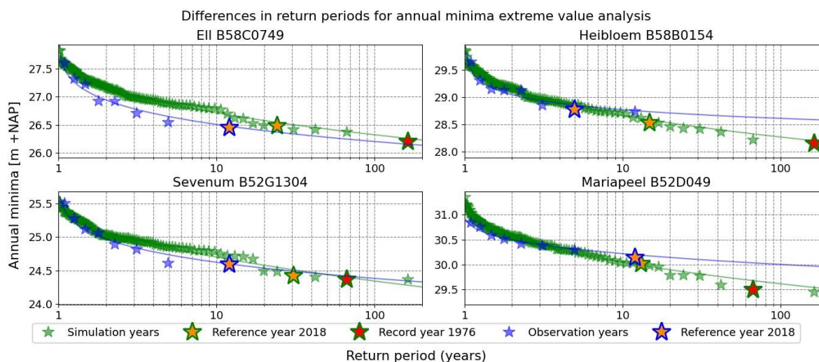
Figure 26: Return periods for annual minima with best fitting extreme value distribution.
