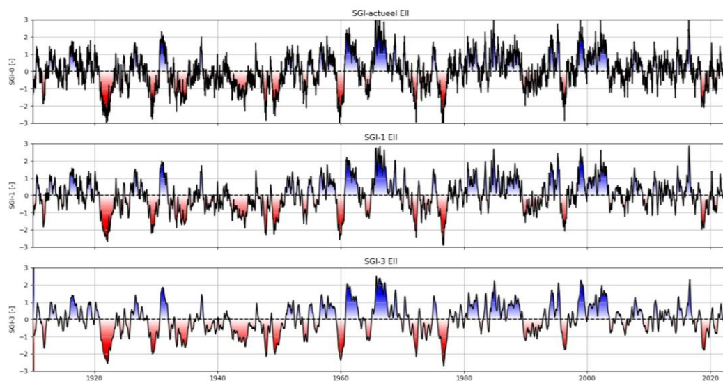
Figure 52: Difference between SGI-0, SGI-1 and SGI-3 for monitoring location Eil.
