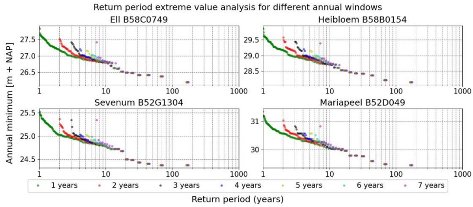
Figure 55: Sensitivity analysis of estimating drought frequency (peak selection in Figure 54)
