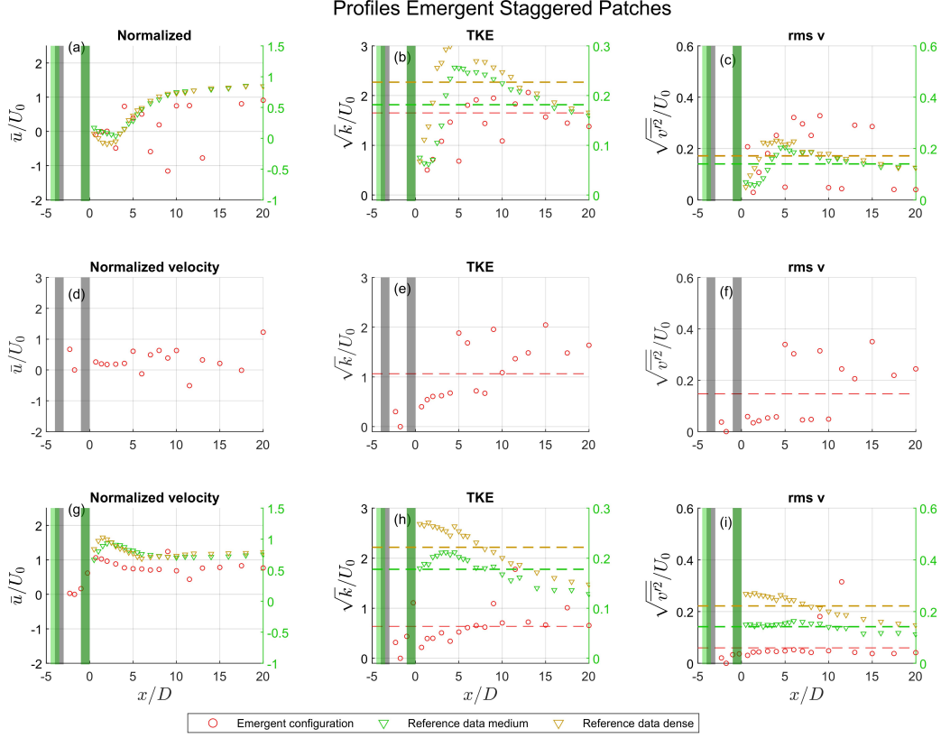
Figure 21: Profiles for three transversal location of emergent configuration: center-line behind upstream, center-line between patches, and center-line behind downstream patch. The normalized mean longitudinal velocity, \bar{u}/U_0 , profiles are shown in subfigures a , d , and g . Normalized Turbulent Kinetic Energy (TKE) longitudinal profiles are shown in subfigures b , e , and h . Lastly, the remaining sub-figures show normalized square-root turbulent kinetic energy, \sqrt{k}/U_0 , in sub-figures c , f , and i . Reference study data is plotted of medium and dense patches spaced longitudinally 2.5D and transversely 0.5D , indicated by green bars. The longitudinal patch positions of the experiments conducted are indicated by grey bars.
