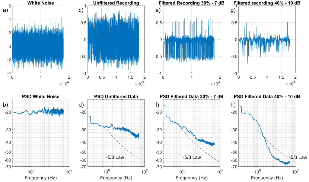
Figure 14: Effect of recording and filters on white noise and power spectral density (PSD) analysis. In a and b respectively, a white noise signal and power spectral analysis of the white noise are shown. In c and d , the same is shown for an unfiltered recording of a water flow. Again, the same is shown in e and f , but for the filtered data with a 30% correlation - 7 dB filter threshold before despiking was done. Lastly, the same is shown in g and h , but for the filtered data with a 40% correlation - 10 dB filter threshold. The dashed line represents the -5/3 law, the natural dissipation of turbulence.
