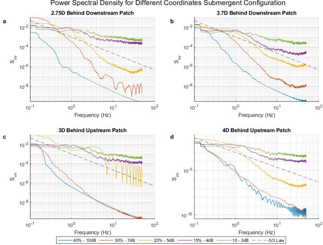
Figure 18: Power spectral densities with various filter thresholds despiking for submerged patches for velocity v . The filters affect how the decay of turbulence will be present in the filtered data set. a and b show power spectral density behind the downstream patch's center line. c and d show the density behind the upstream patch's center line. The legend shows the various filters applied and, additionally, the 5/3 law of dissipation of the turbulence line.
