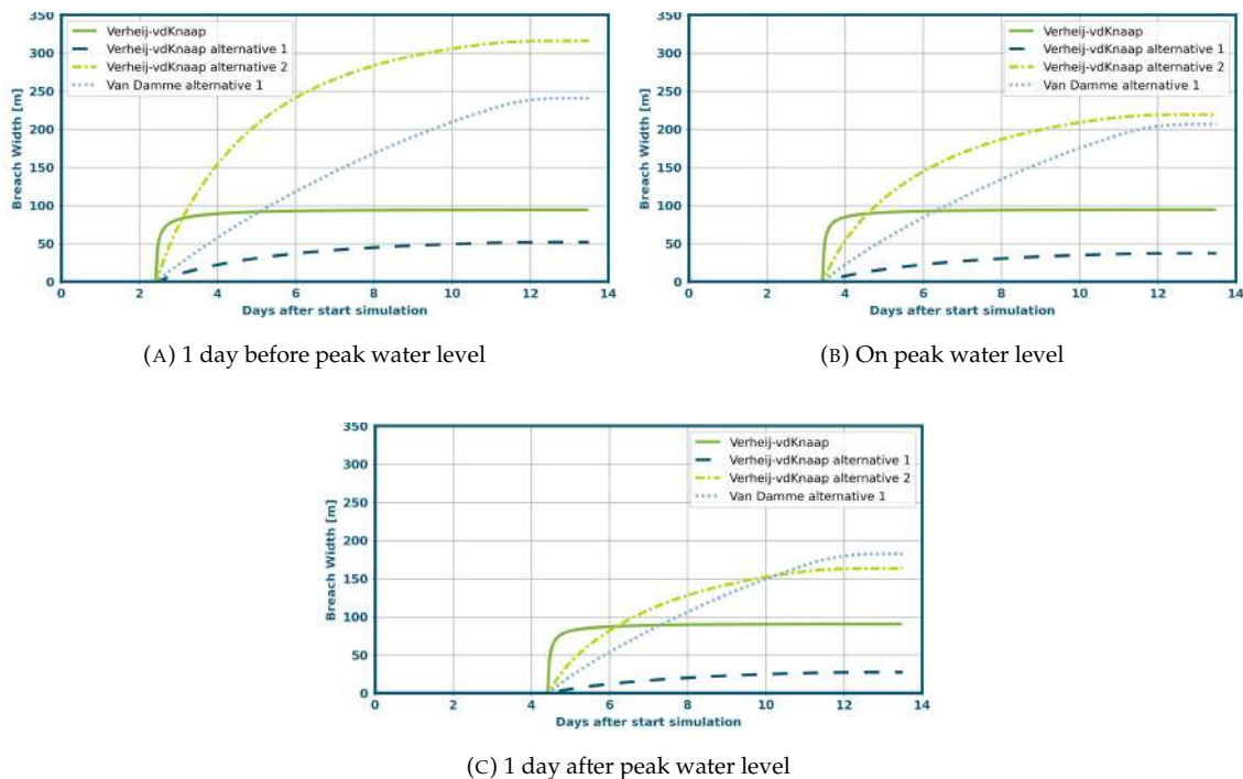
FIGURE 3.9: Breach growth at three different initiation moments
