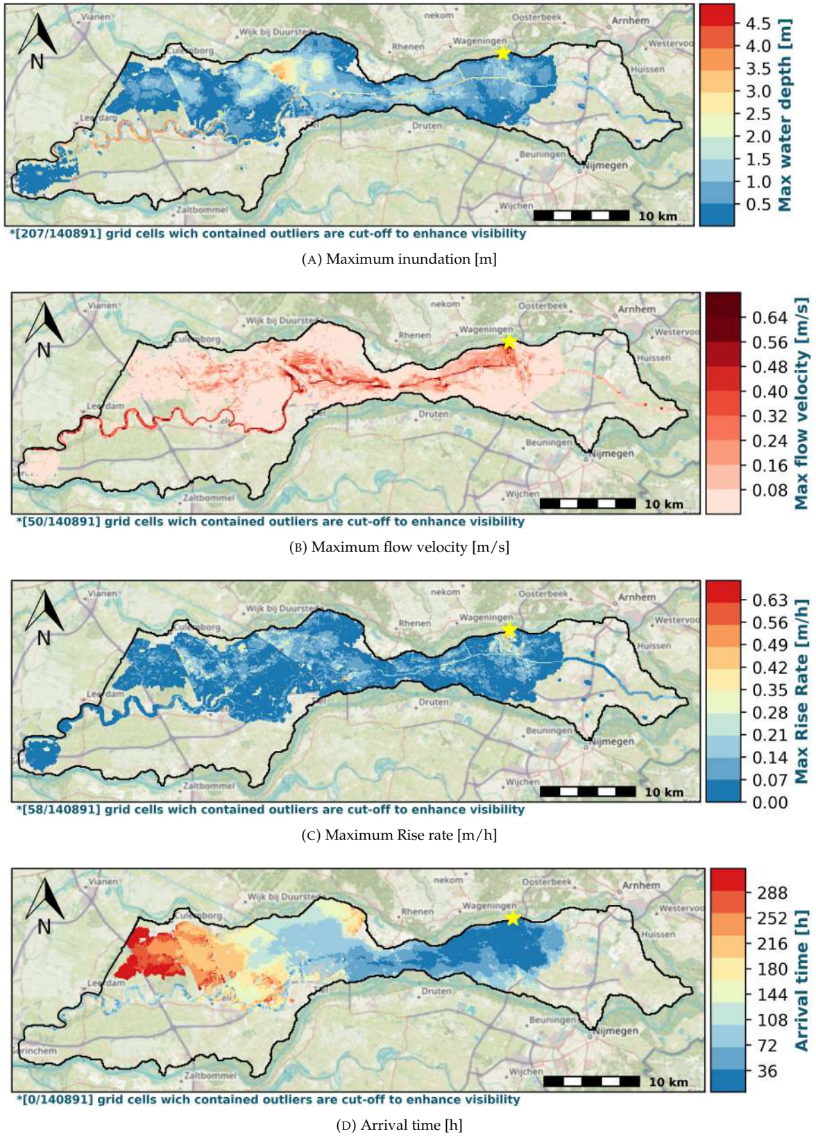
FIGURE C.17: Fixed weir with elevation change model run at Heteren [Yellow star = breach location]
