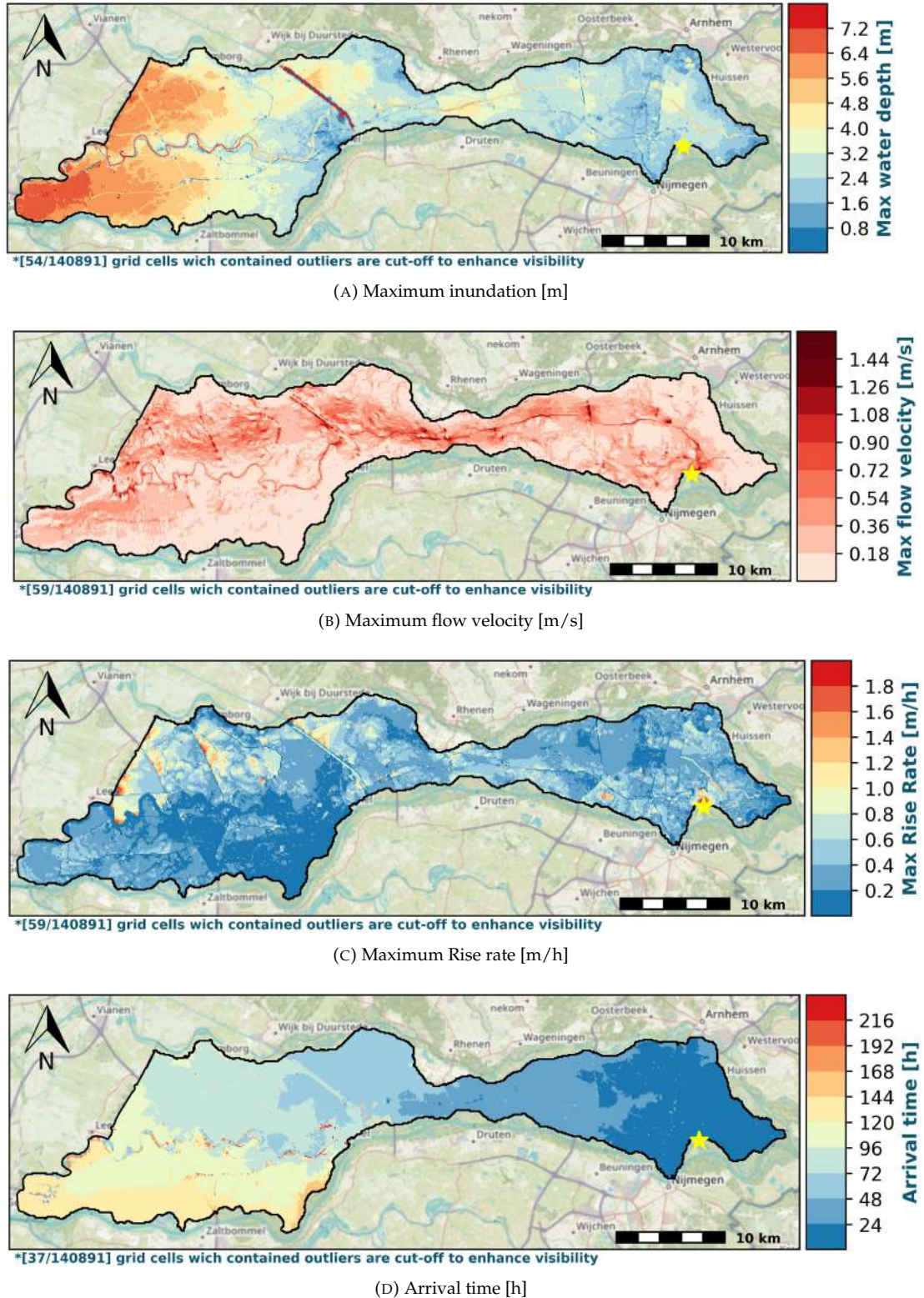
FIGURE C.14: Fixed weir without elevation change Bommel [Yellow star = breach location]
