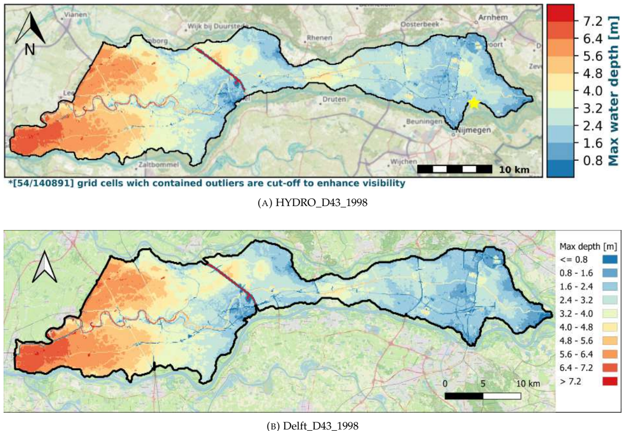
FIGURE 4.1: Maximum inundation depth at Bemmél [Yellow star = Breach location]
