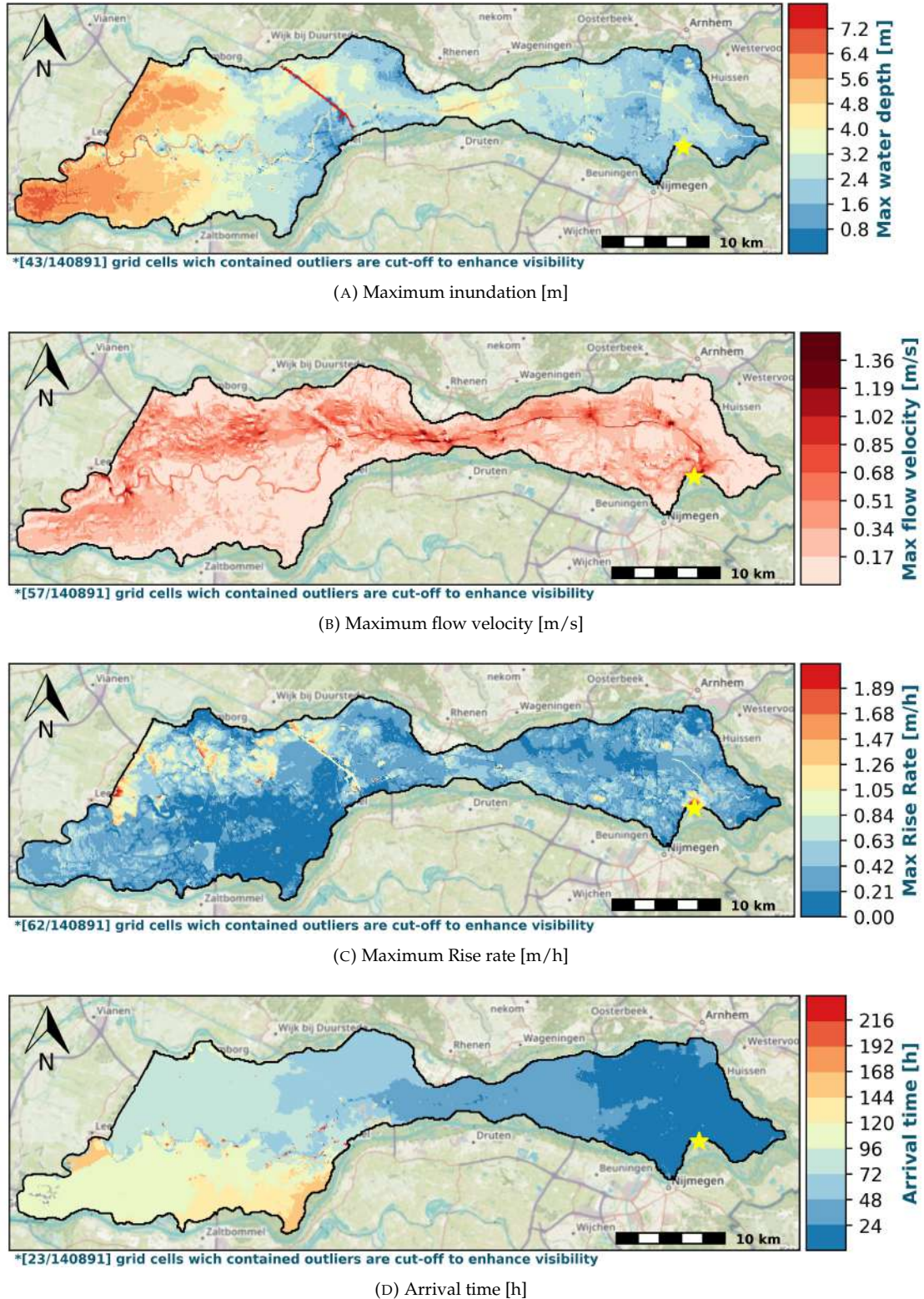
FIGURE C.16: Fixed weir with elevation change at Bommel [Yellow star = breach location]
