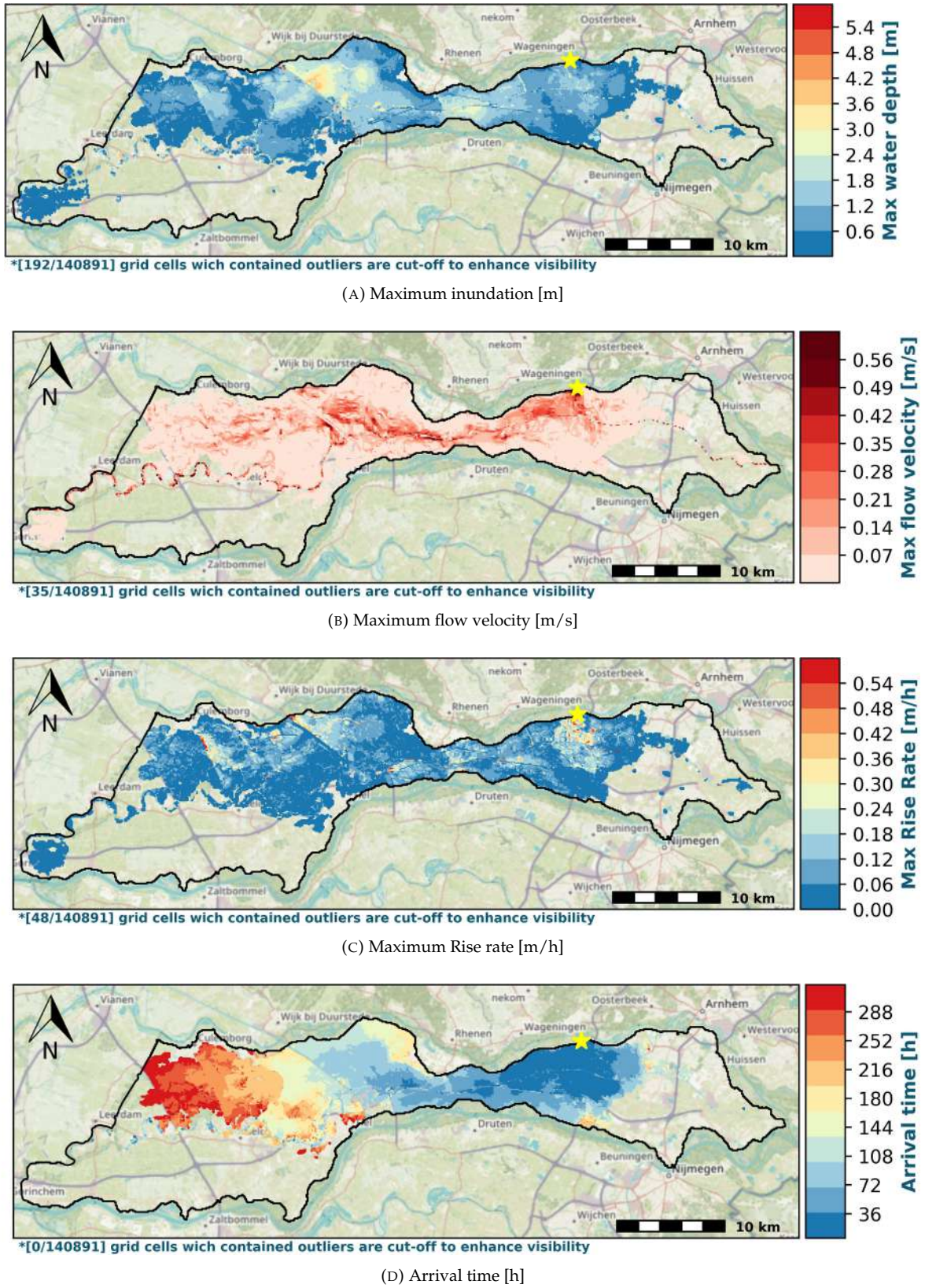
FIGURE C.20: Detailed Linge grid model run at Heteren [Yellow star = breach location]
