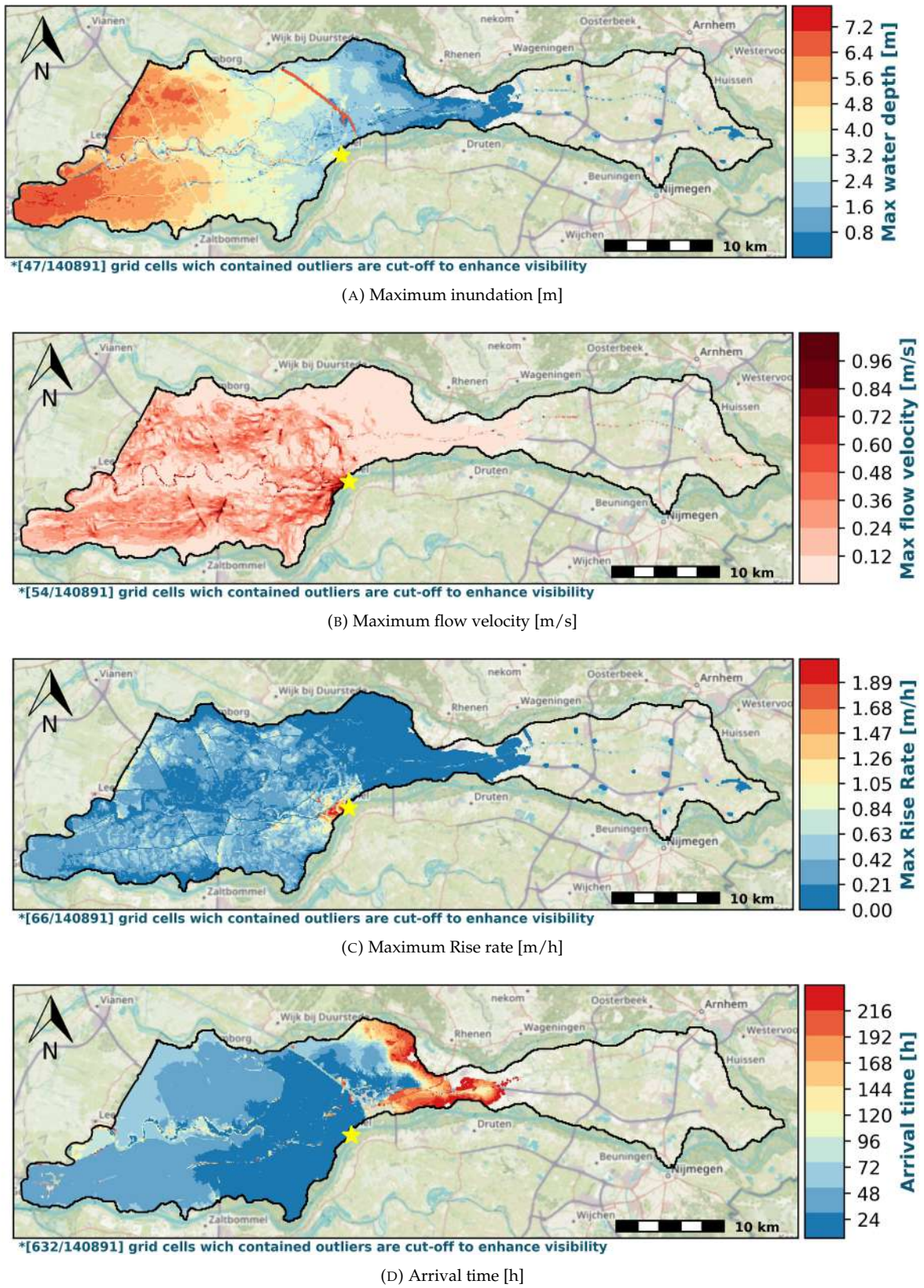
FIGURE C.19: Detailed Linge grid model run at Tiel [Yellow star = breach location]
