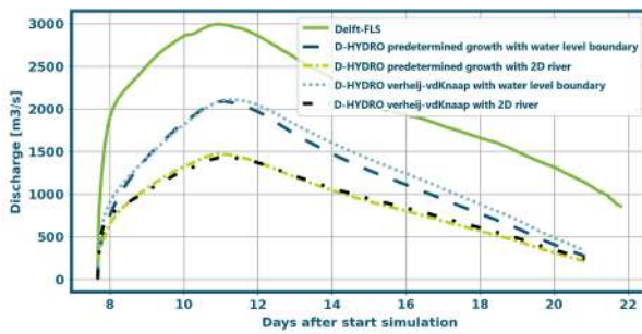
(C) Breach hydrograph at Tiel
