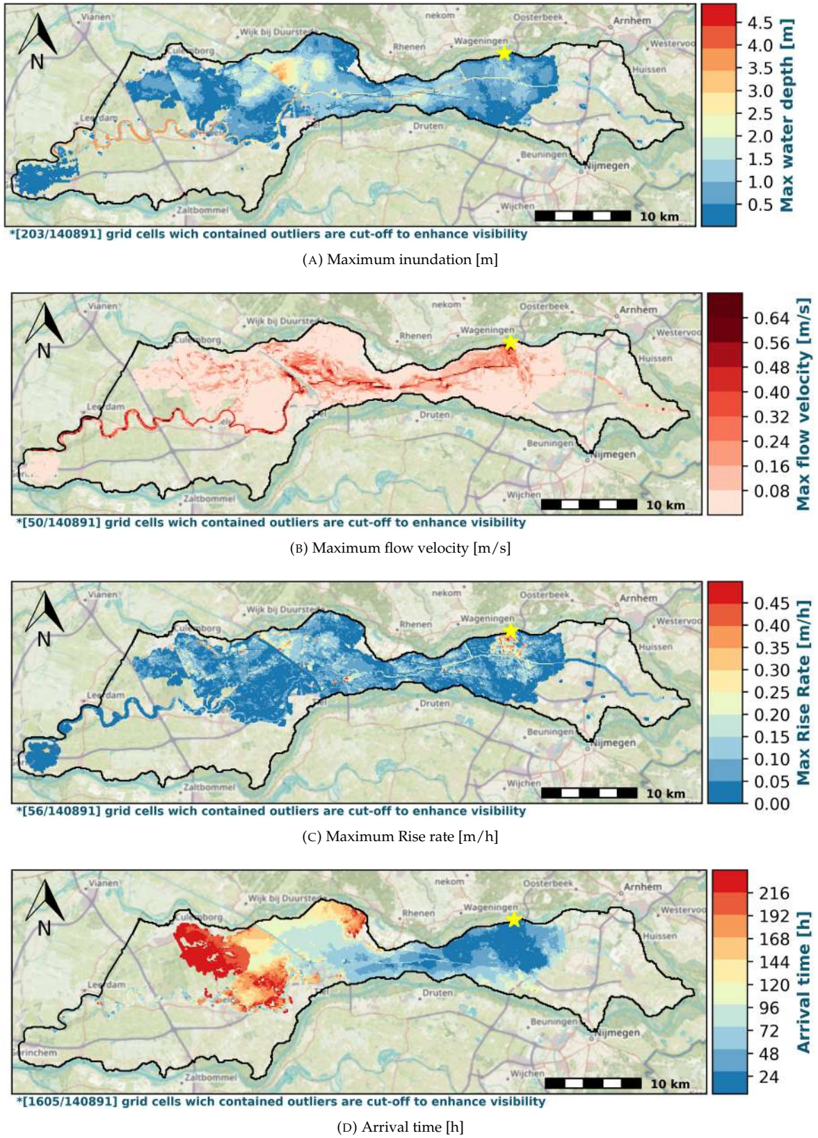
FIGURE C.15: Fixed weir without elevation change model run at Heteren [Yellow star = breach location]
