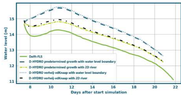
(B) Upstream water level at Bemmel
