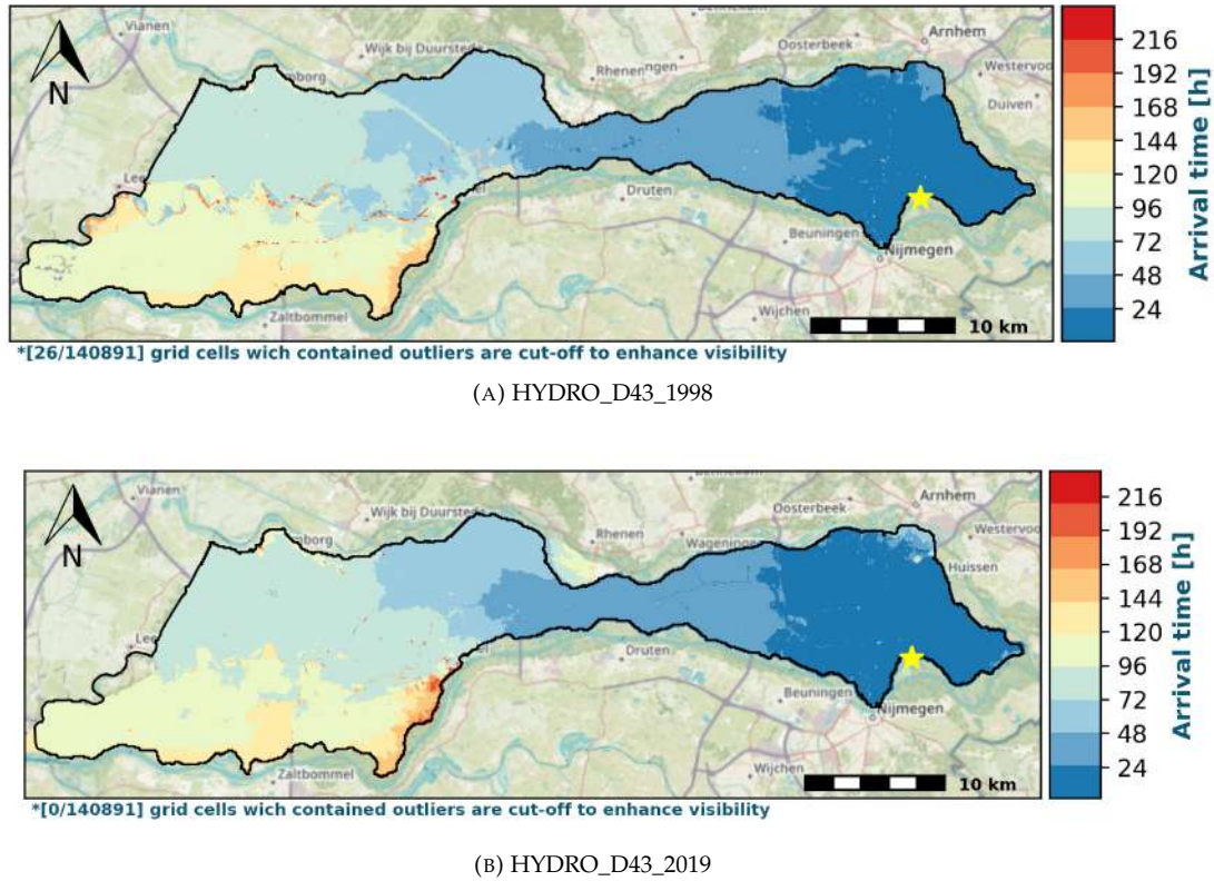
FIGURE 4.5: Arrival time at Bommel [Yellow star = breach location]
