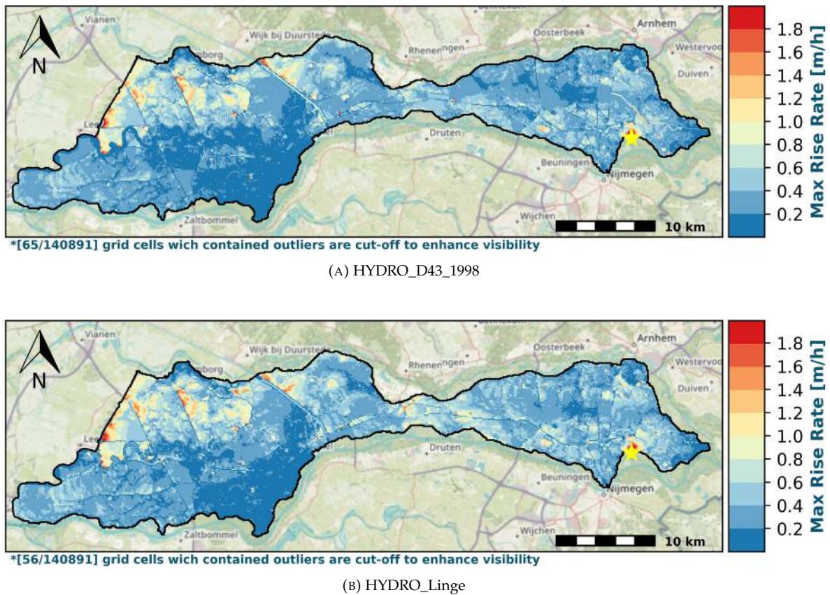
FIGURE 4.14: Maximum rise rate dike breach at Bemmel [Yellow star = breach location]
