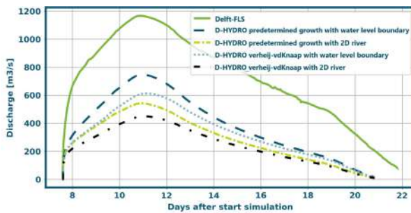
(E) Breach hydrograph at Heteren
