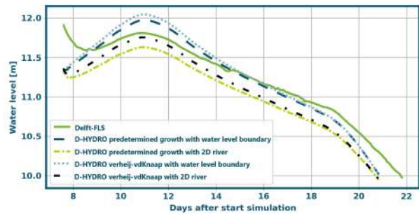
(F) Upstream water level at Heteren
