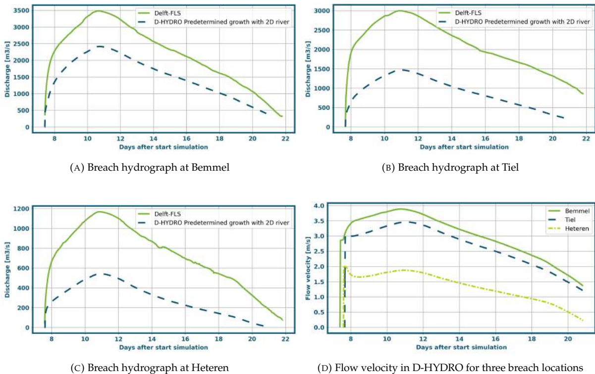
FIGURE 3.1: Delft-FLS vs D-HYDRO
