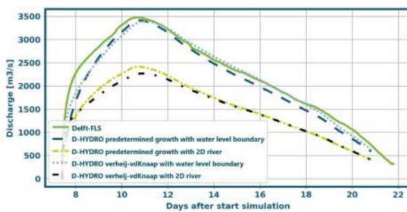
(A) Breach hydrograph at Bemmel
