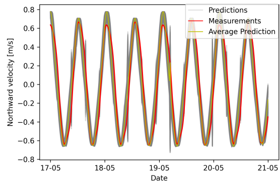
Figure 32: Predicted and measured northward velocities in the model domain for the WC method. For each of the grid cells in the model domain, the predicted northward velocities are plotted in grey. The yellow line shows the predicted velocities at the average measurement location.
