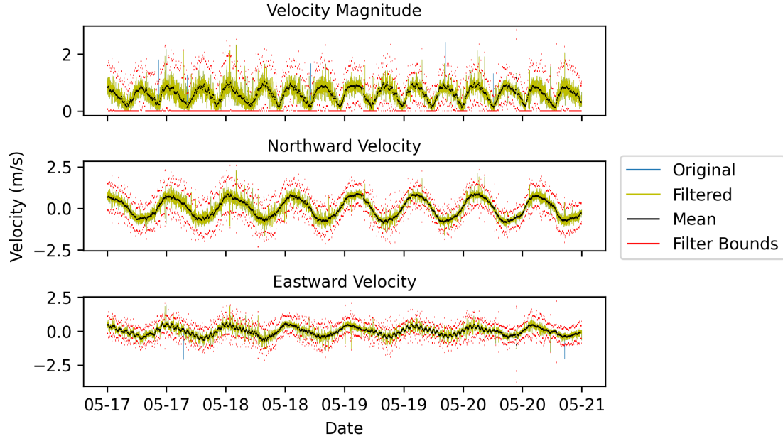
Figure 49: Filtering process for a complete time series based on 6 standard deviations of with respect to the mean velocity for overlapping batches of 10 minutes at a water depth of 7 meters.
