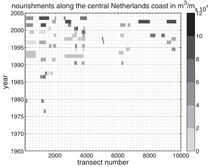
Figure 3.2: Nourishment location, frequency and intensity.
