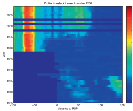
Figure 4.12: Dune evolution at transect 1260.
