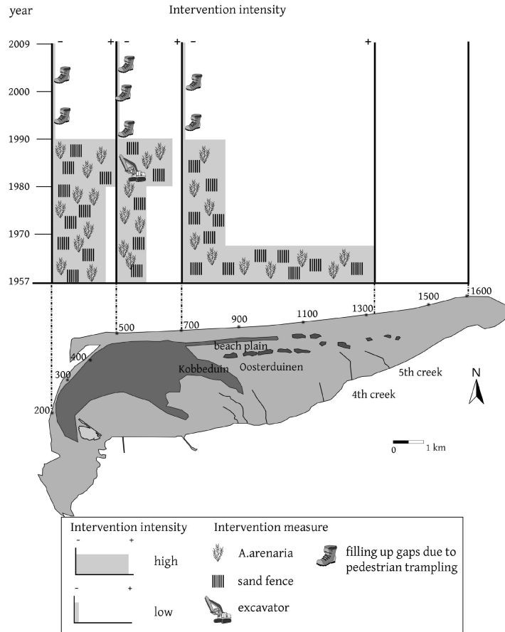
Figure 4.3: Intervention measures and intensities from 1957 to 2009. The numbers refer to the transect locations (Jarkus profile measurement locations).
