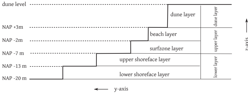
Figure 1.4: PONTOS model schematization. NAP is the Netherlands' Ordnance Datum, which corresponds approximately to mean sea level.
