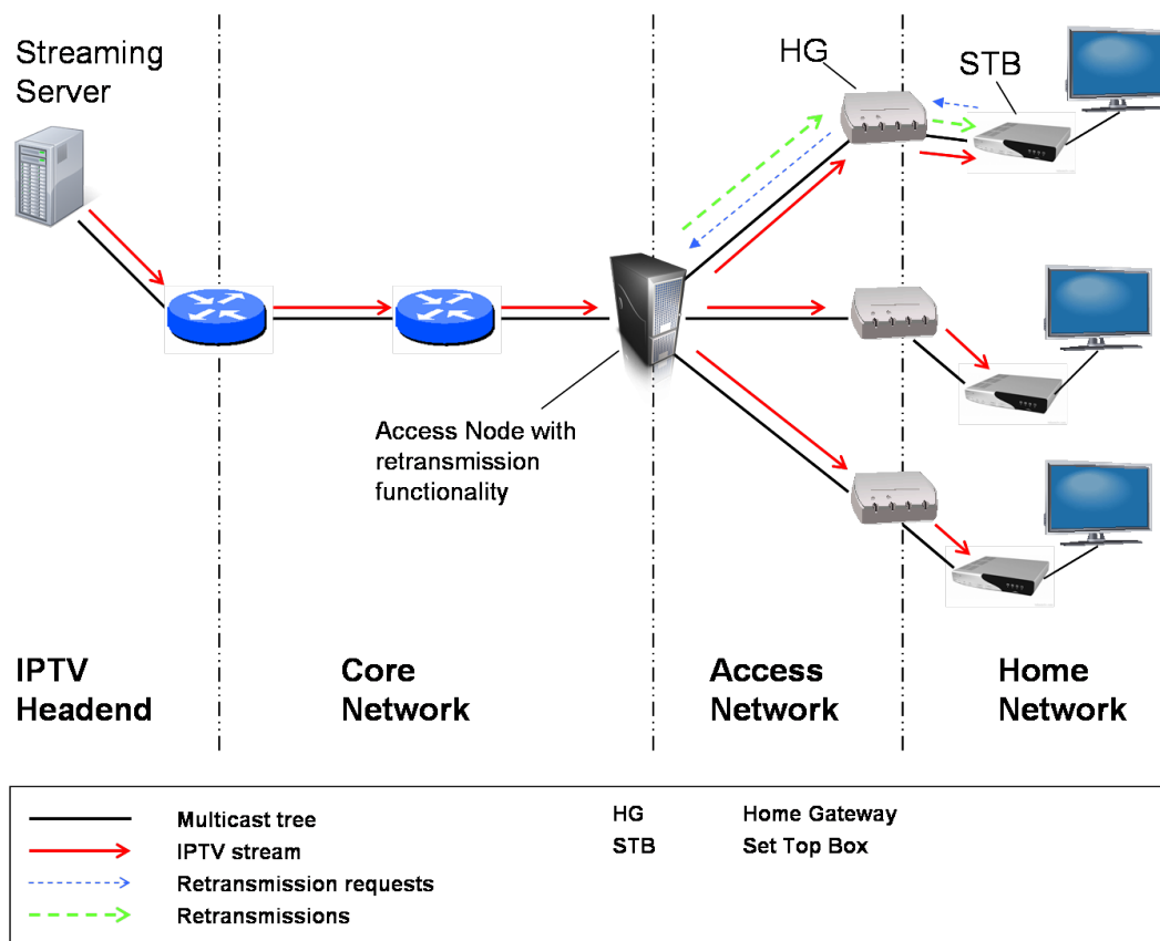
Figure 3.2: IPTV distribution network with retransmission functionality provided by the Access Node
