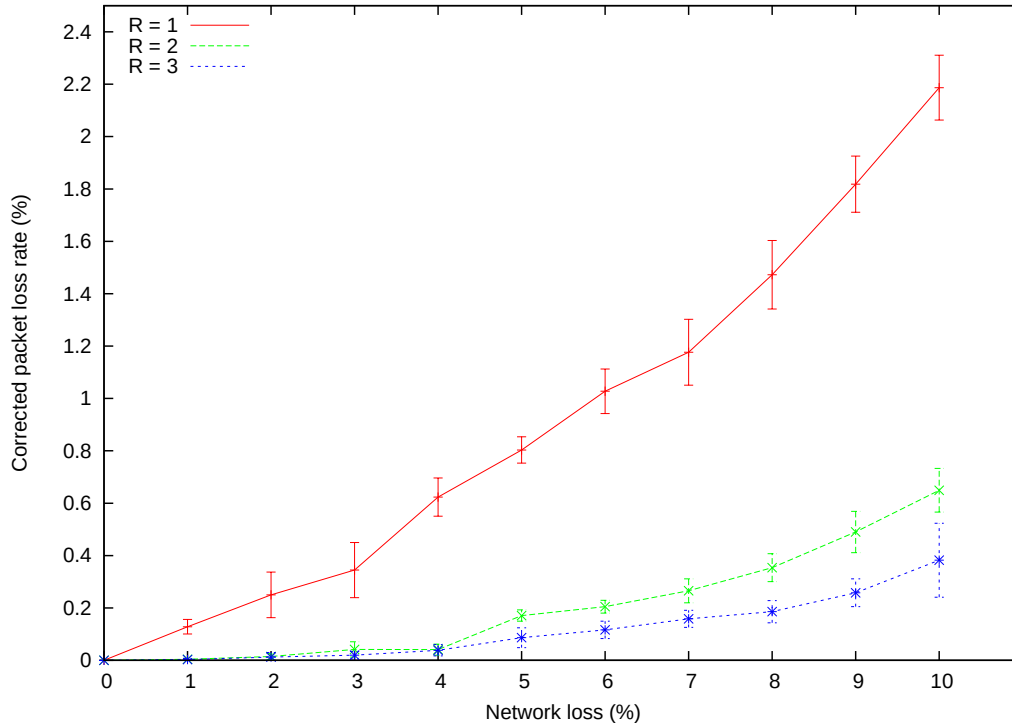
Figure 5.17: Error recovery performance for correlated packet loss with a refined retransmission timeout mechanism
