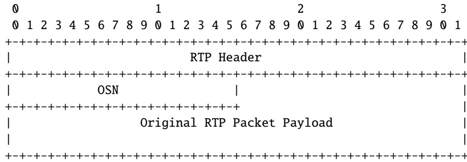
Figure 4.7: RTP Retransmission Payload Format
