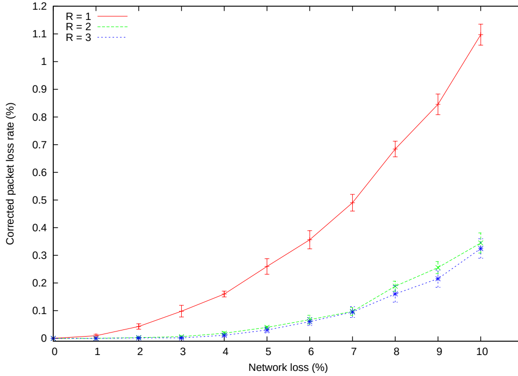
Figure 5.11: Error recovery performance for uncorrelated packet loss for one ( R=1 ), two ( R=2 ) or three ( R=3 ) allowed retransmission attempts
