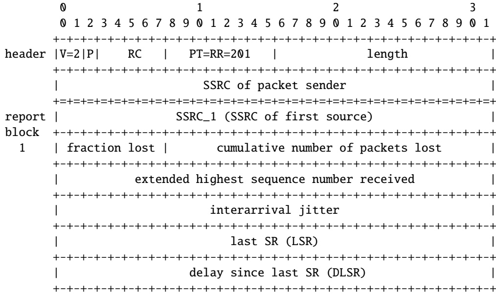
Figure 2.5: RTCP packet header with receiver report
