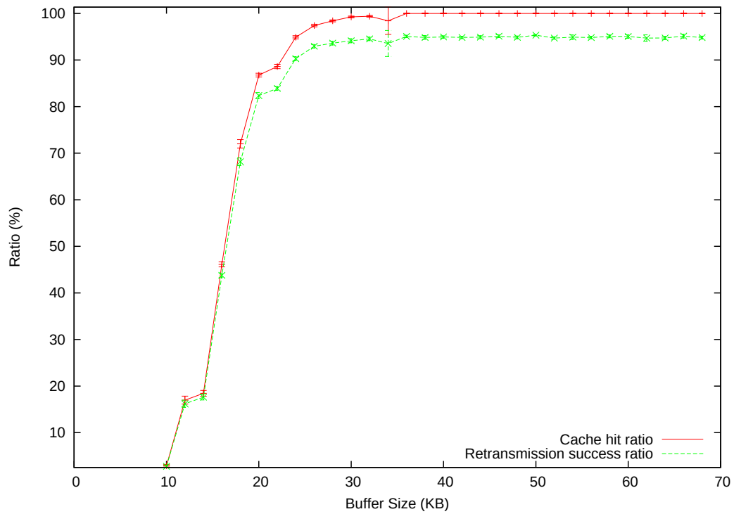
Figure 5.6: Buffer dimensioning Retransmission Cache with one retransmission attempt
