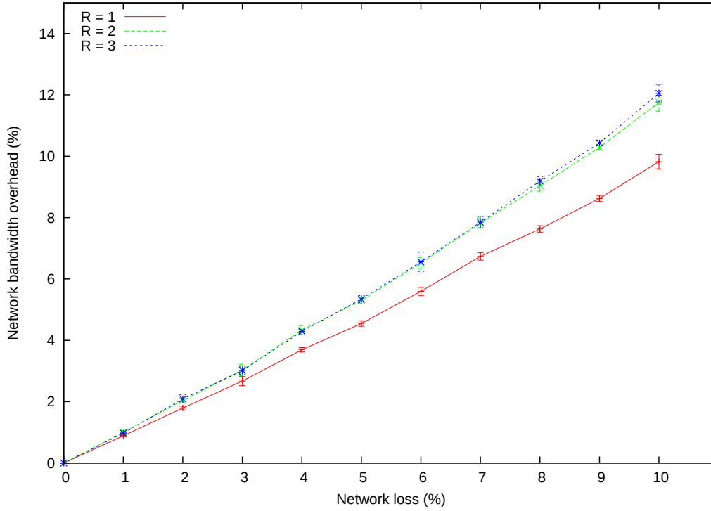
Figure 5.15: Retransmission bandwidth, burst network loss
