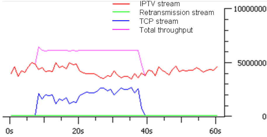
Figure 5.20: Congestion trace - without retransmissions
