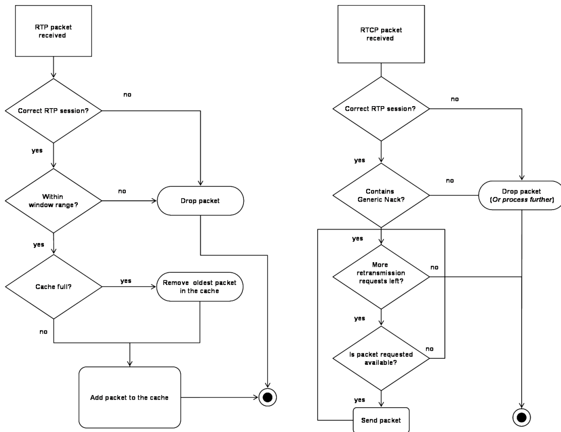
Figure 4.9: Retransmission Cache activity diagram
