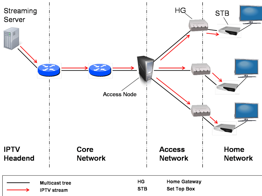
Figure 3.1: IPTV distribution network
