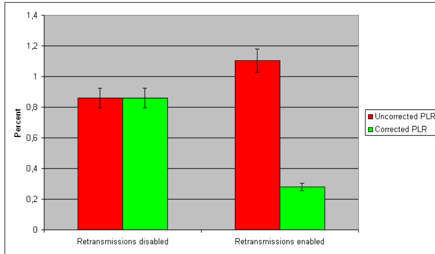
Figure 5.22: Retransmission in congested network
