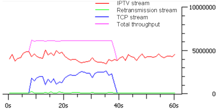
Figure 5.21: Congestion trace - with retransmissions
