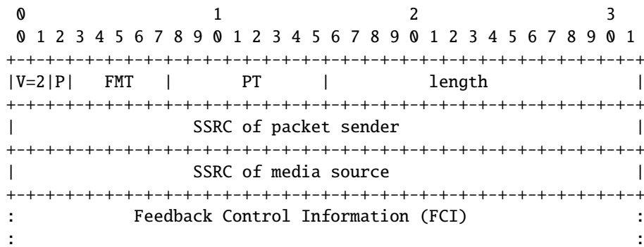
Figure 4.5: Common packet format for feedback messages
