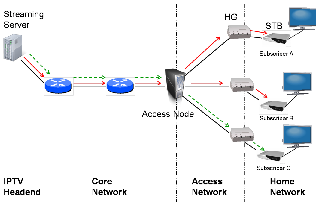
Figure 2.3: A IPTV distribution network for broadcast TV, with two IPTV streams transmitted to different users
