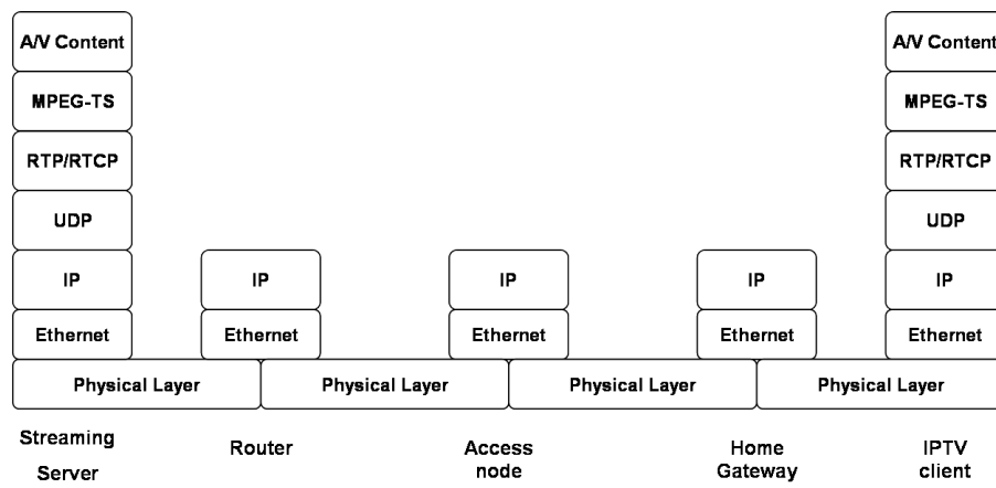
Figure 4.1: Multicast IPTV distribution protocol stack with RTP and MPEG-TS
