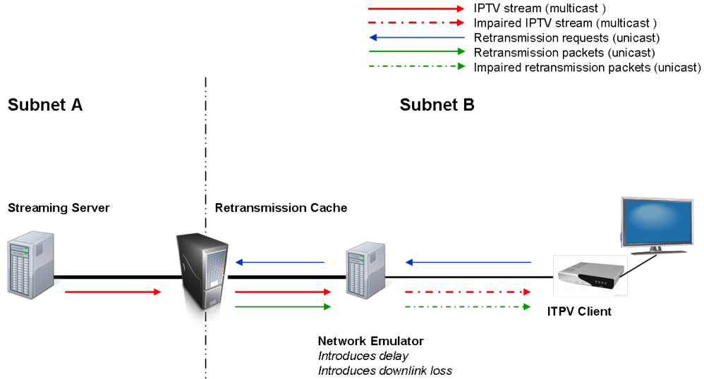
Figure 5.5: Network with an uncongested access link
