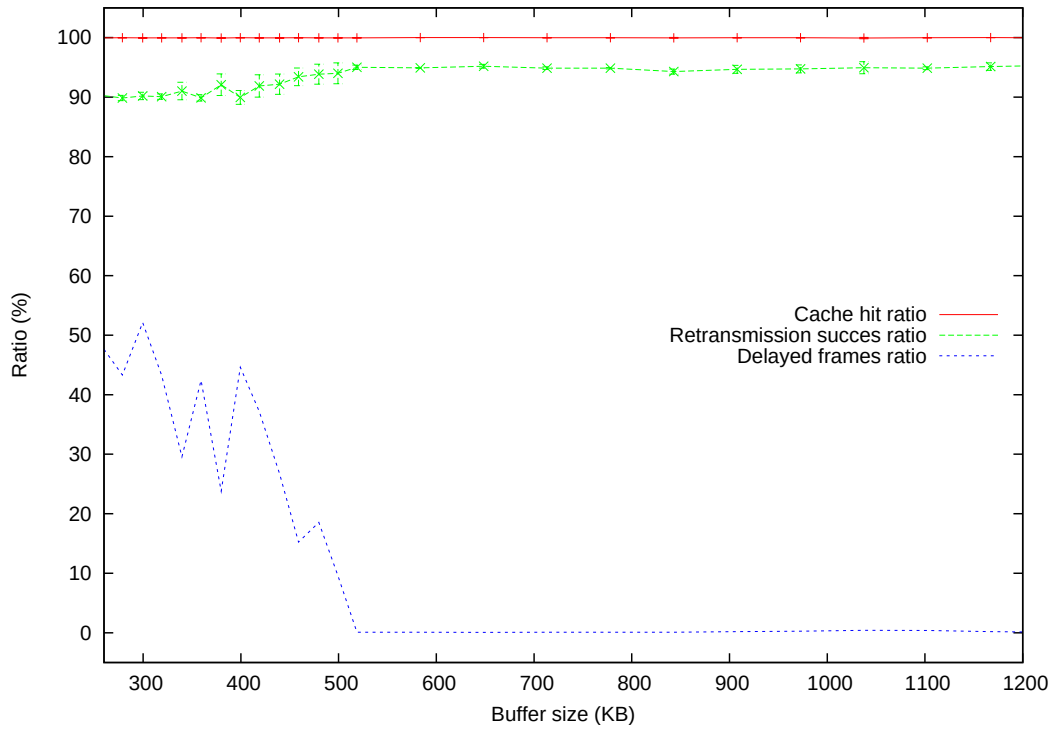
Figure 5.8: Buffer dimensioning IPTV Client, one retransmission attempt
