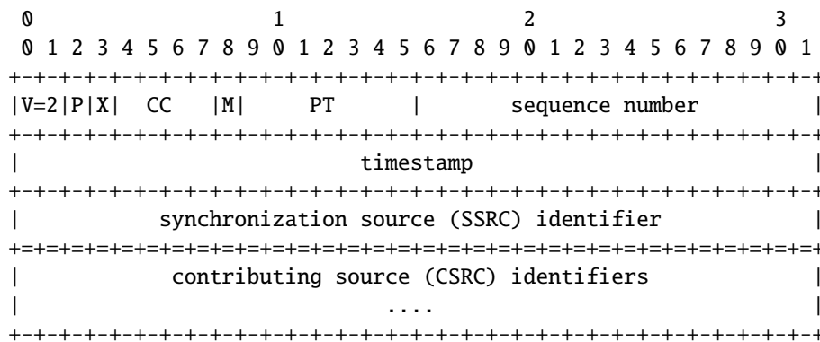
Figure 2.4: RTP packet header
