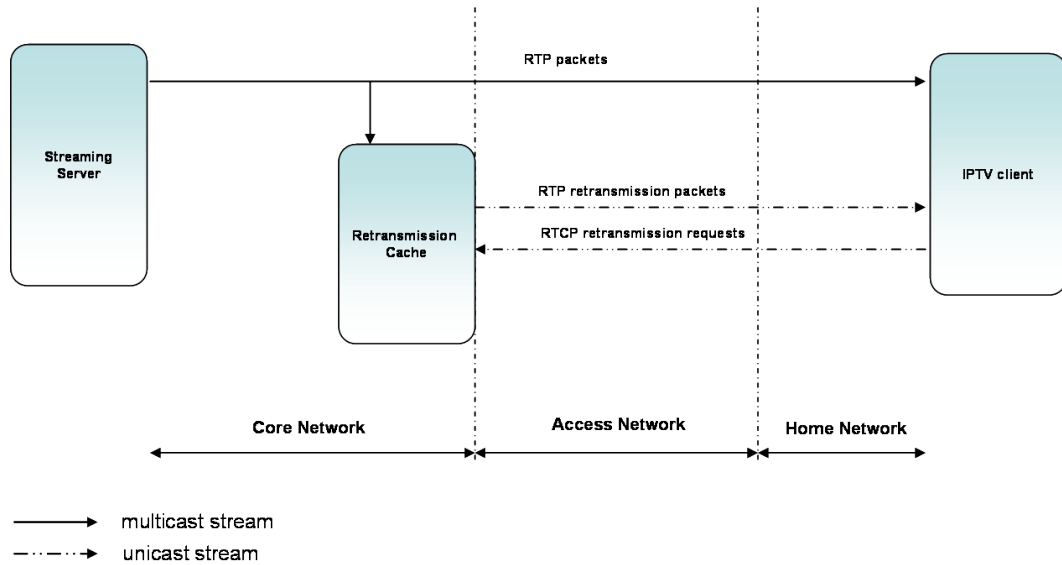
Figure 4.3: IPTV Retransmission Components
