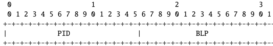
Figure 4.6: RTCP Generic NACK message
