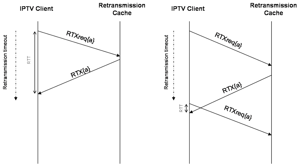
Figure 4.8: Retransmission RTT estimation (correct and incorrect)
