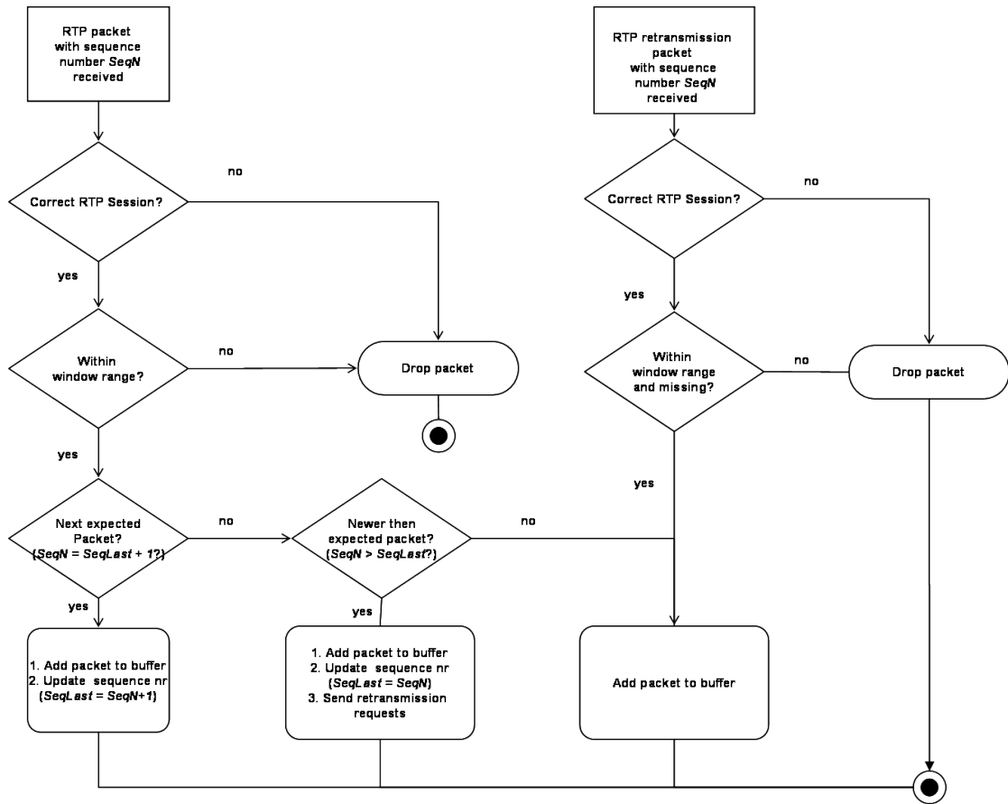
Figure 4.10: IPTV Client activity diagram
