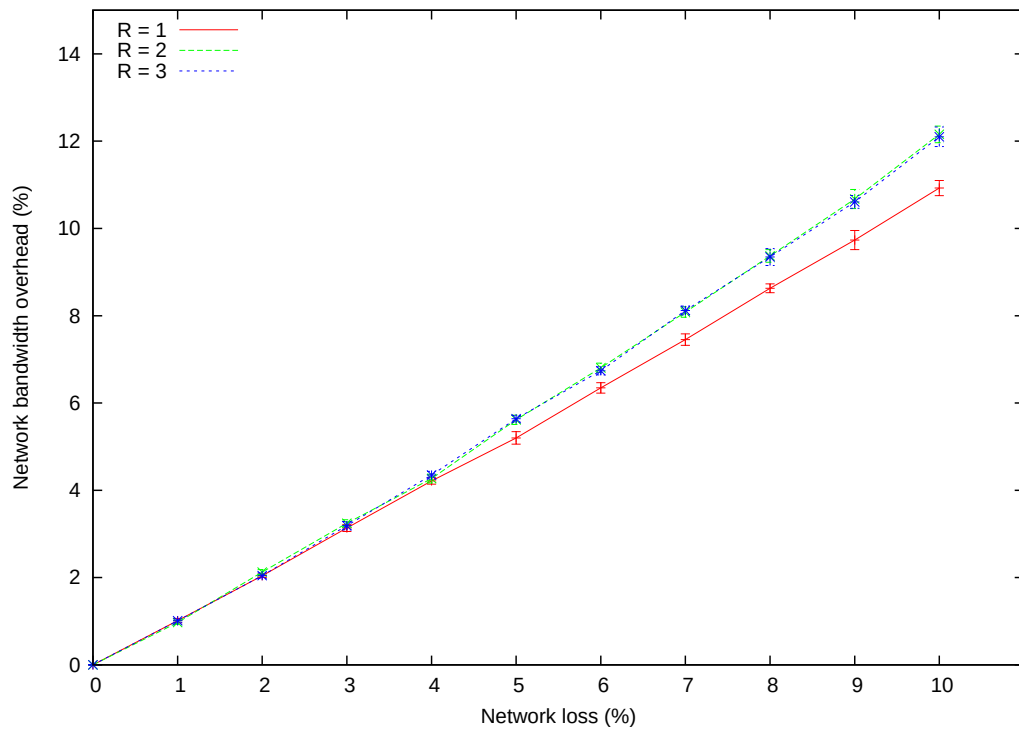
Figure 5.12: Retransmission Bandwidth overhead for uncorrelated packet loss for one ( R=1 ), two ( R=2 ) or three ( R=3 ) allowed retransmission attempts
