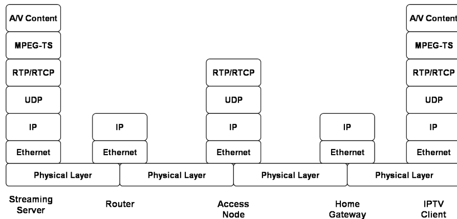
Figure 4.2: Multicast IPTV distribution protocol stack with packet retransmission
