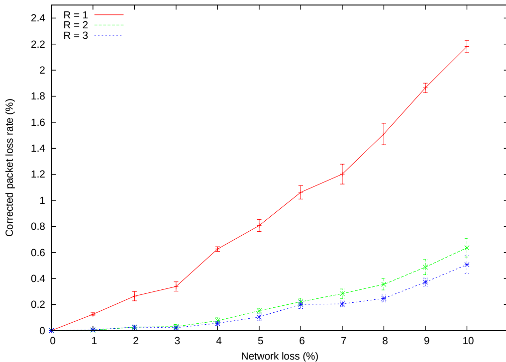
Figure 5.14: Error recovery performance for correlated packet loss for one ( R=1 ), two ( R=2 ) or three ( R=3 ) allowed retransmission attempts
