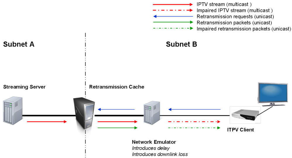
Figure 5.10: Test setup network - Uncongested Access Link
