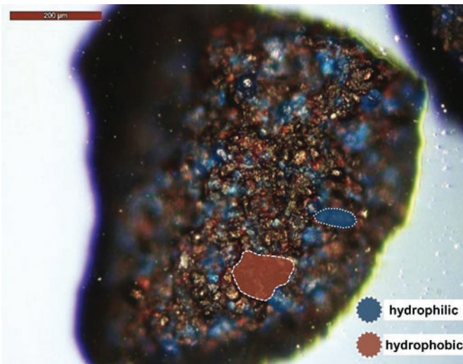
Pd/alumina catalyst with hydrophobic and hydrophilic domains
