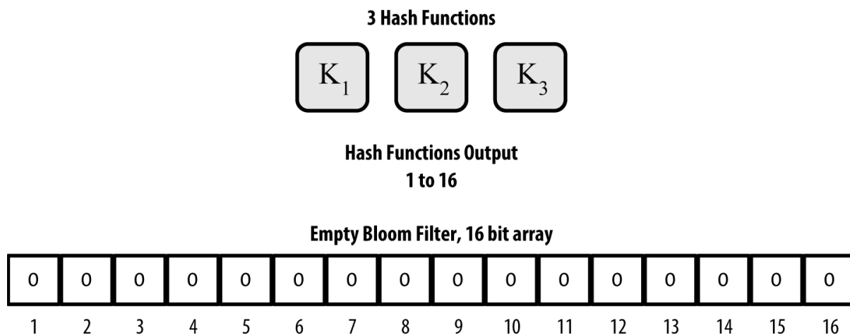
Figure 8. An example of a simplistic bloom filter, with a 16-bit field and three hash functions
