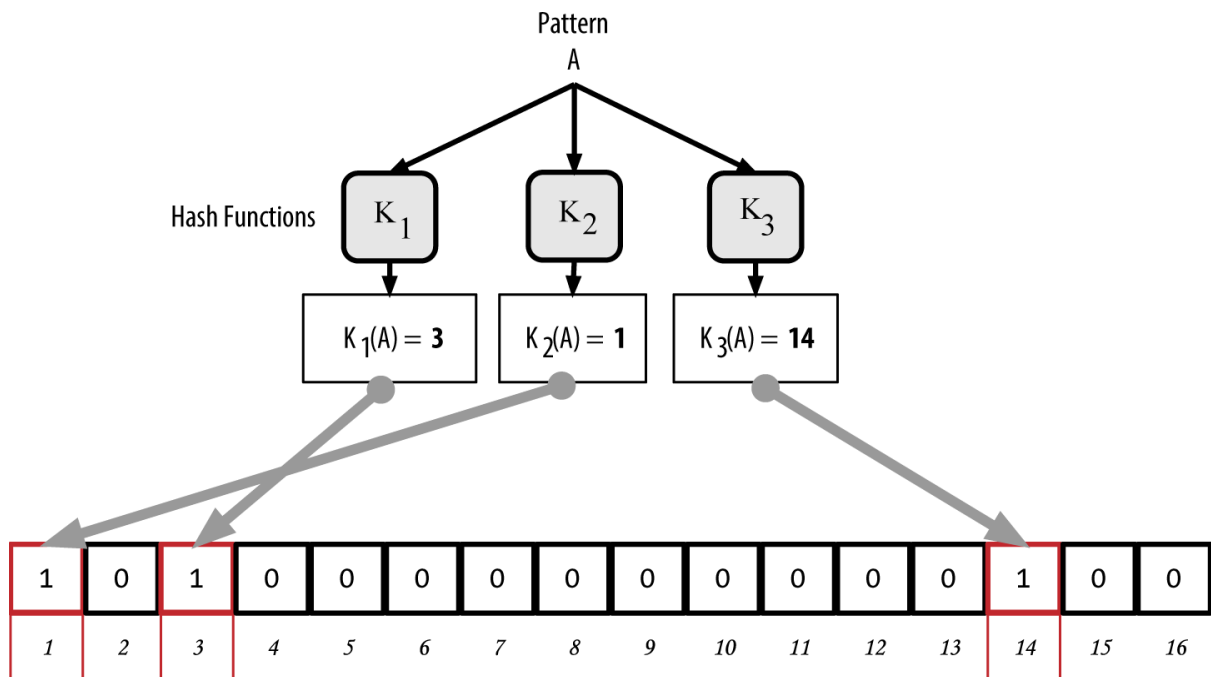
Figure 9. Adding a pattern "A" to our simple bloom filter
