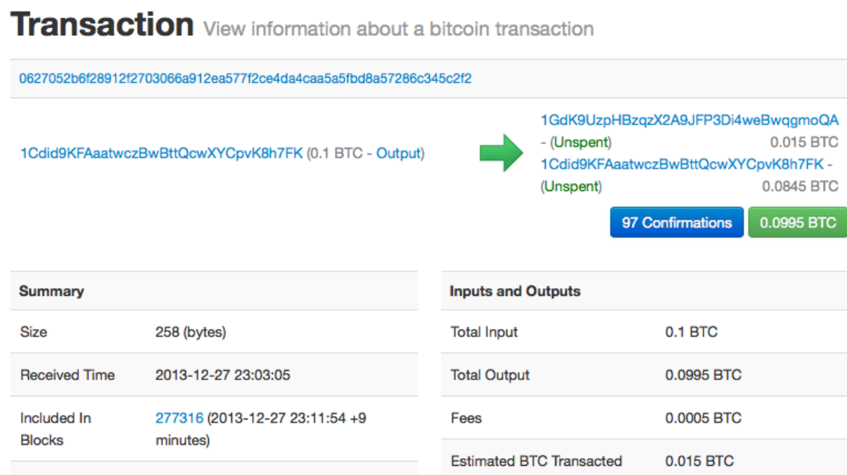
Figure 1. Alice's transaction to Bob's Cafe
