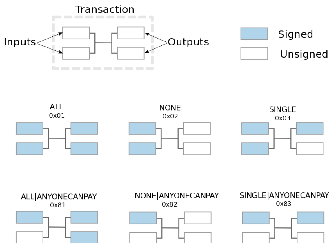
Figure 8. Summary of different sighash combinations
