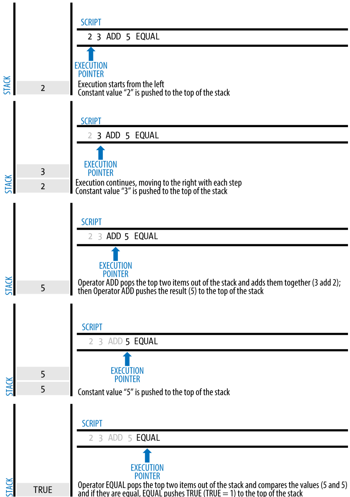
Figure 5. Bitcoin's script validation doing simple math
