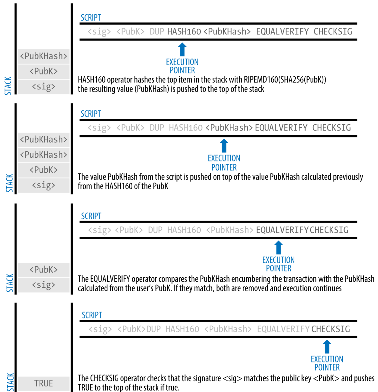
Figure 7. Evaluating a script for a P2PKH transaction (part 2 of 2)
