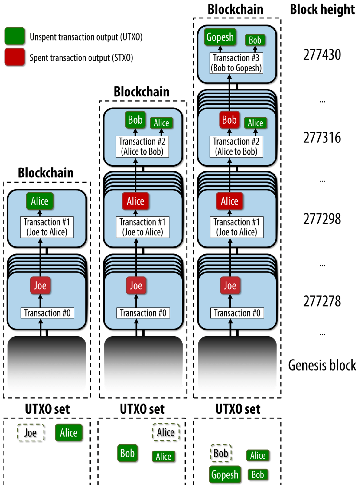
Figure 2. Transaction chain from Joe to Gopesh being built on the blockchain
