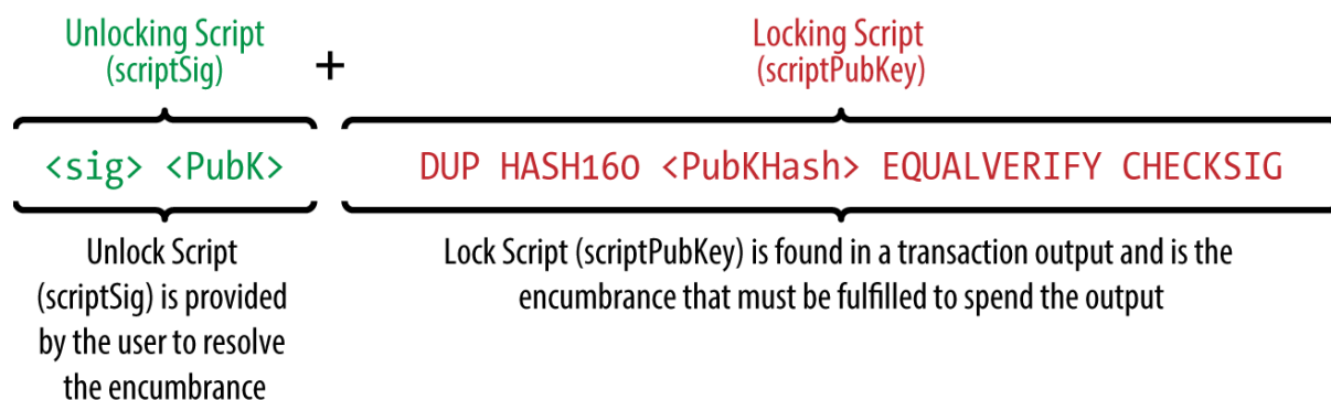
Figure 4. Combining scriptSig and scriptPubKey to evaluate a transaction script
