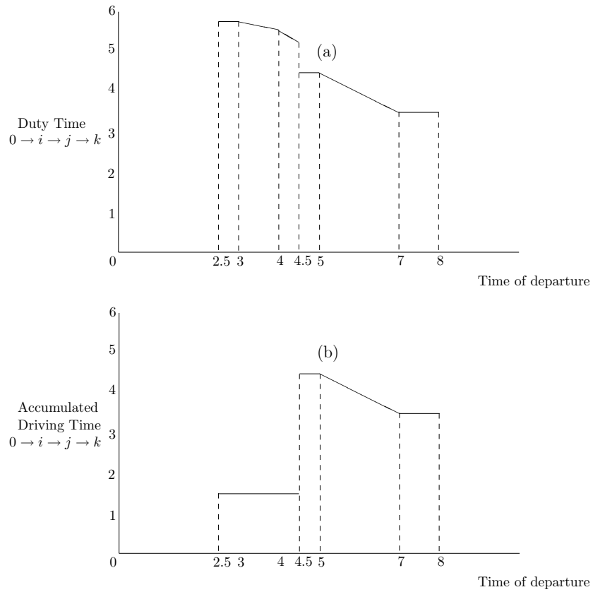
Figure 3: duty time records with time windows and breaks: (a) duty times route 0 \rightarrow i \rightarrow j \rightarrow k , (b) accumulated driving times route 0 \rightarrow i \rightarrow j \rightarrow k
