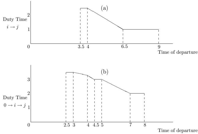
Figure 2: duty time records with time windows: (a) duty times route i \rightarrow j , (b) duty times route 0 \rightarrow i \rightarrow j
