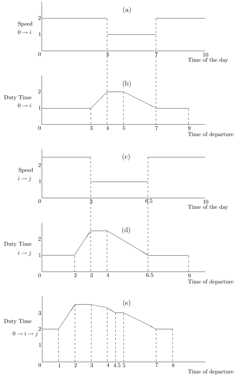
Figure 1: (a) speeds route 0 \rightarrow i , (b) duty times route 0 \rightarrow i , (c) speeds route i \rightarrow j , (d) duty times route i \rightarrow j , (e) duty times route 0 \rightarrow i \rightarrow j .
