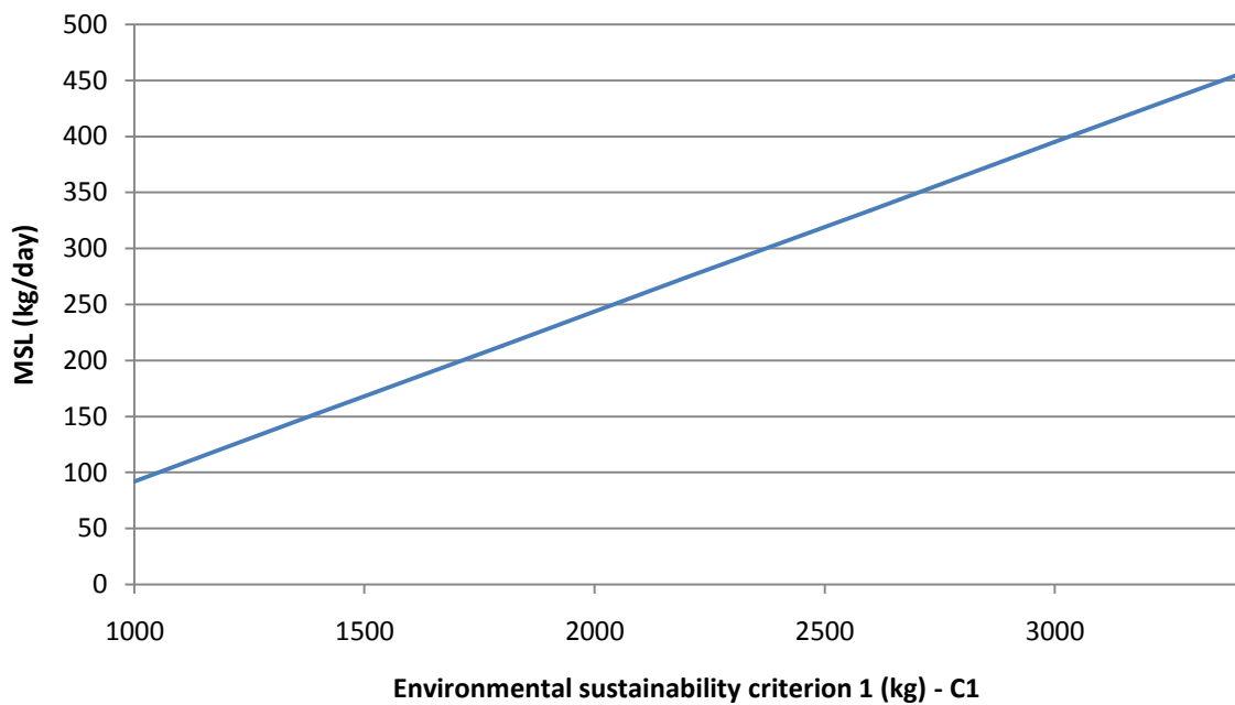
Figure 47: MSL related to variability of C1
