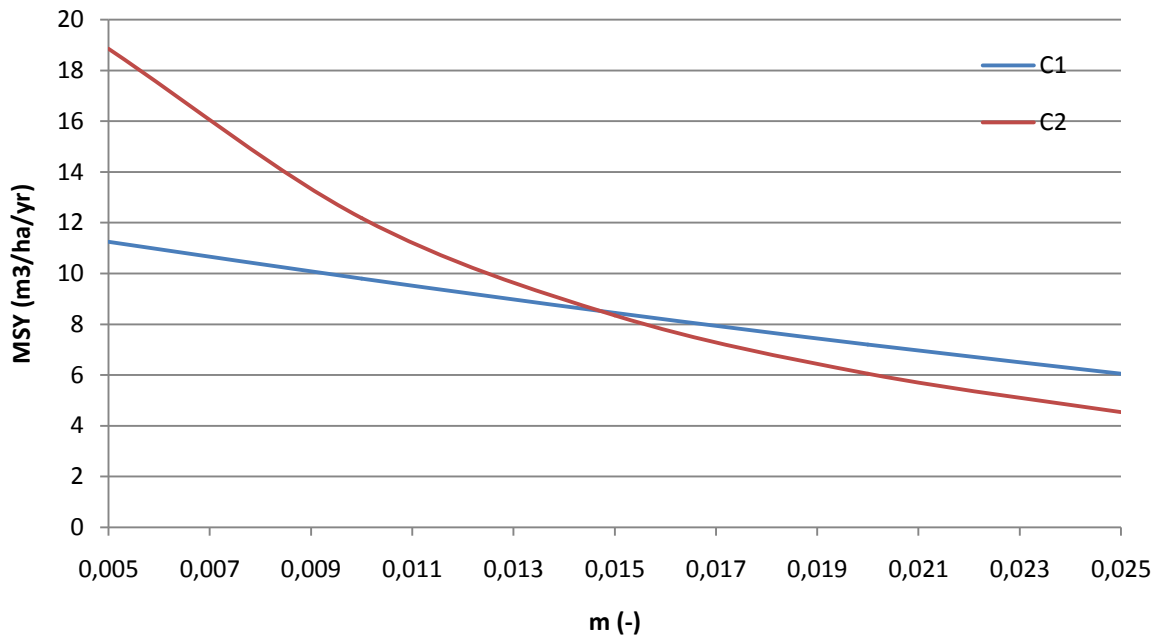
Figure 27: MSY related to variability in mortality rate
