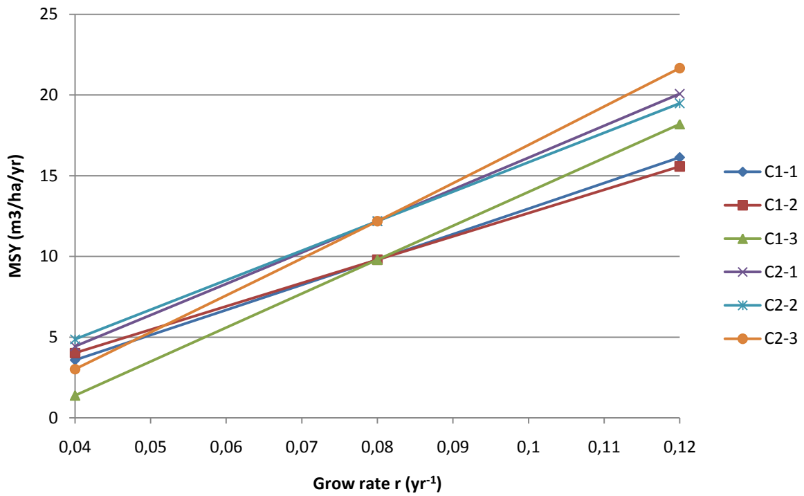
Figure 61: Influence of different types of criteria on the MSY for changing biomass regeneration capacities
