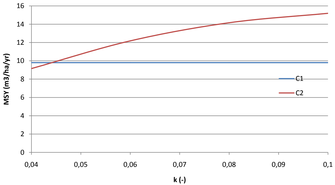
Figure 29: MSY related to variability of the decomposition rate
