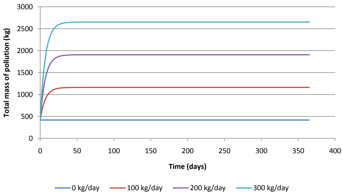
Figure 40: Relation between mass of pollution and load rates
