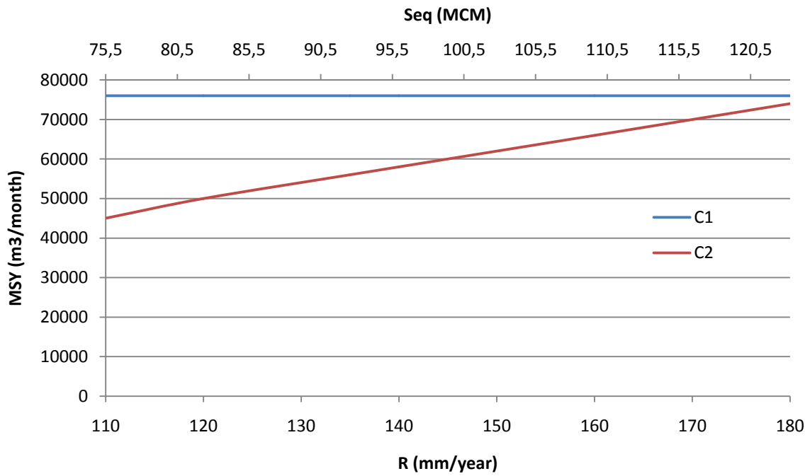
Figure 8: MSY related to variability of recharge
