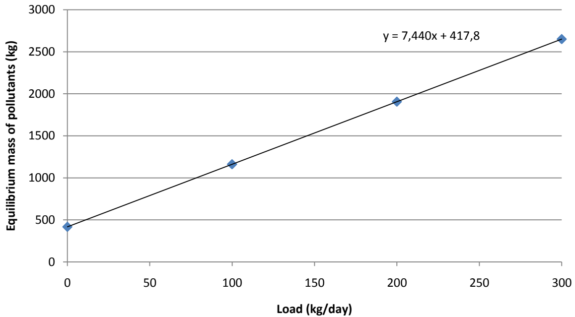
Figure 41: Relation between equilibrium amount mass of pollution and load rate
