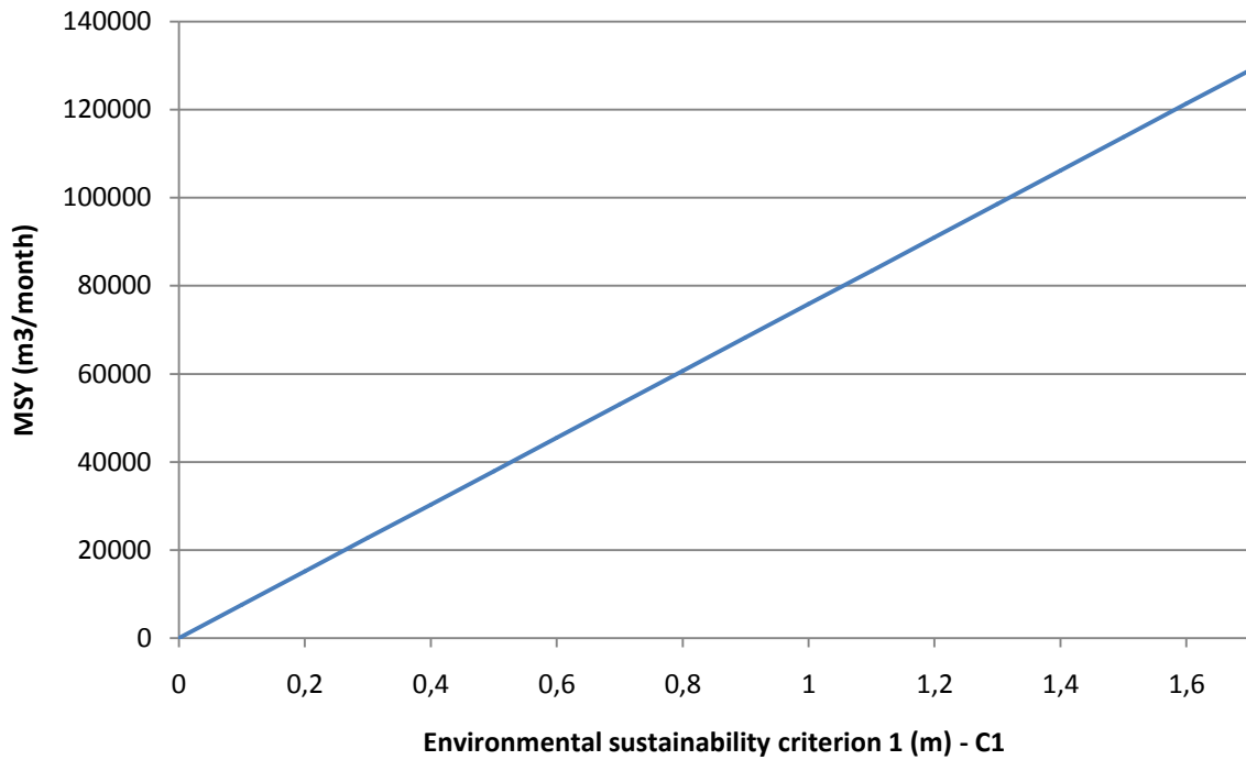
Figure 12: MSY related to variability of C1
