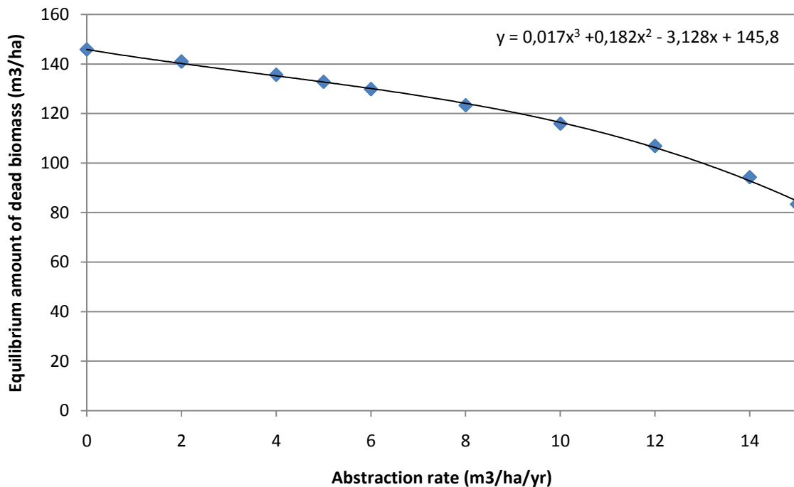
Figure 25: Relation between the equilibrium volume of dead biomass and the abstraction intensity
