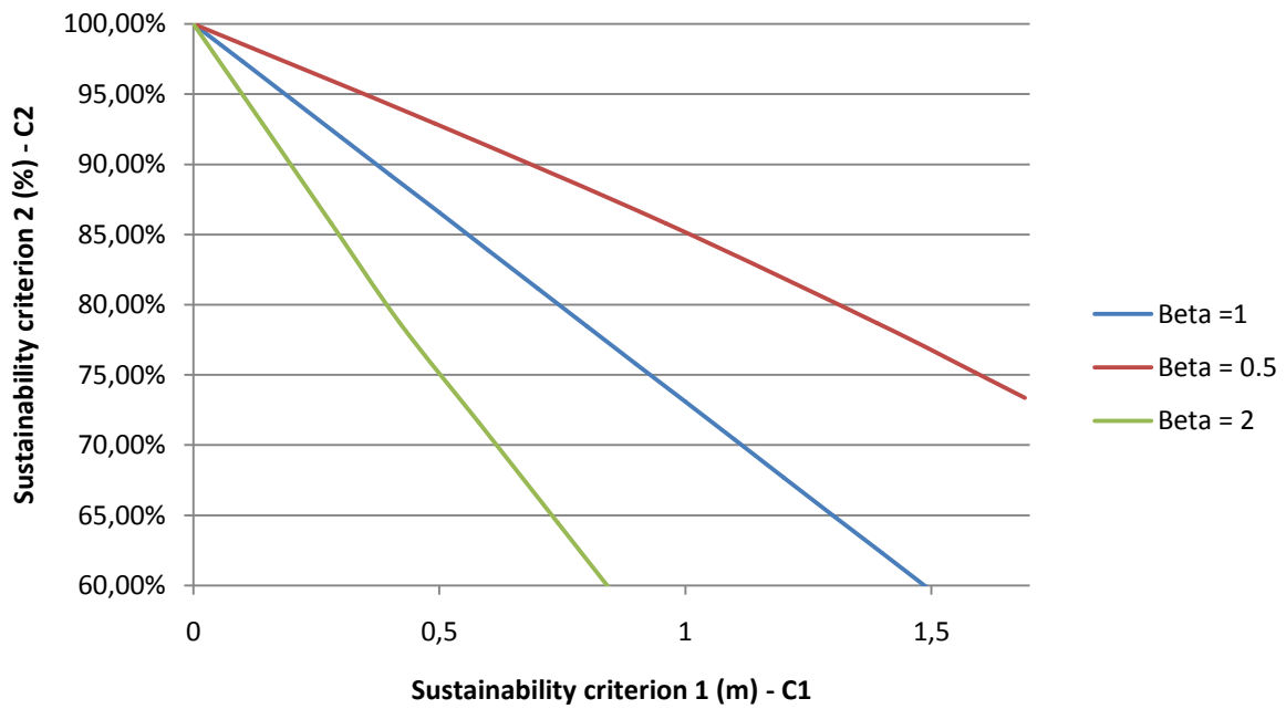
Figure 18: Relation between C1 and C2 for varying beta values
