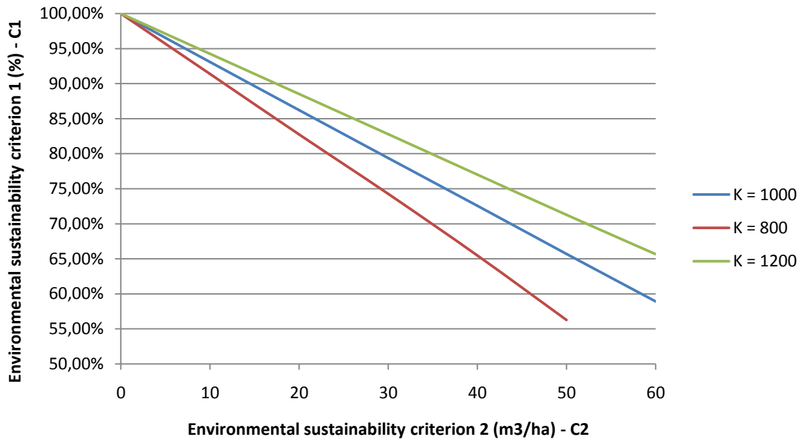
Figure 37: Relation between C1 and C2 for varying carrying capacities
