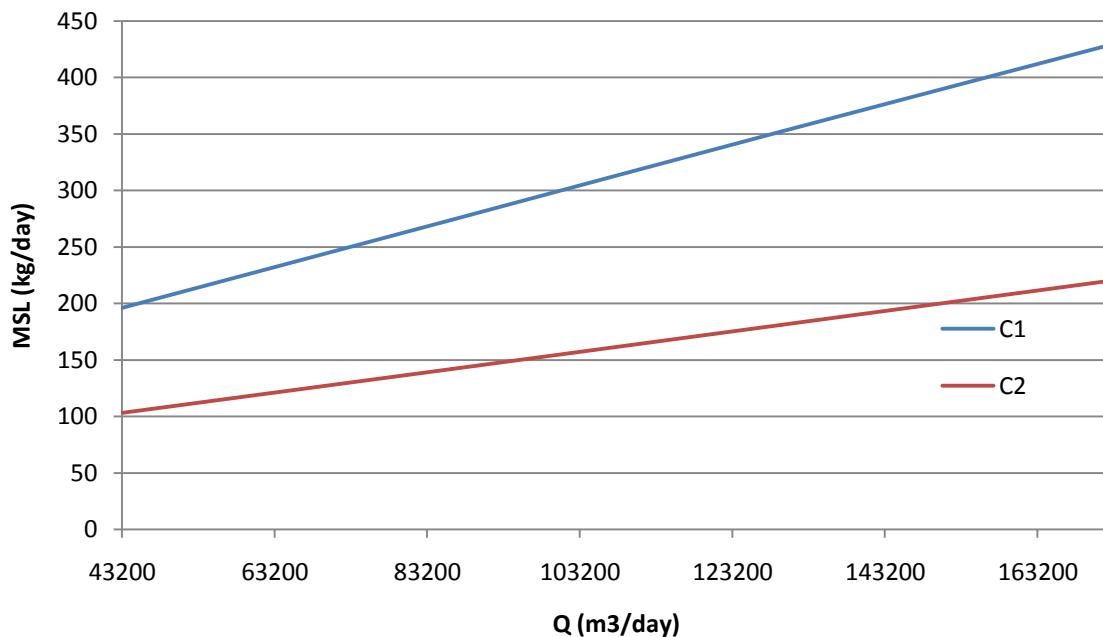
Figure 43: MSL related to variability in discharge
