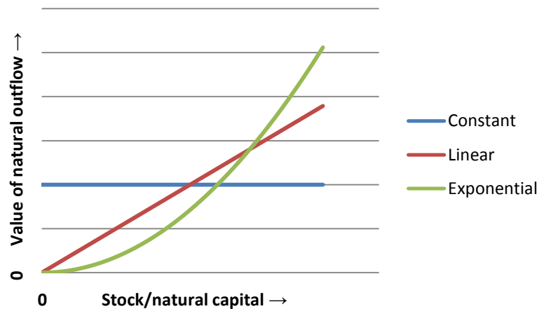
Figure 58: Outflow behavior of environmental systems
