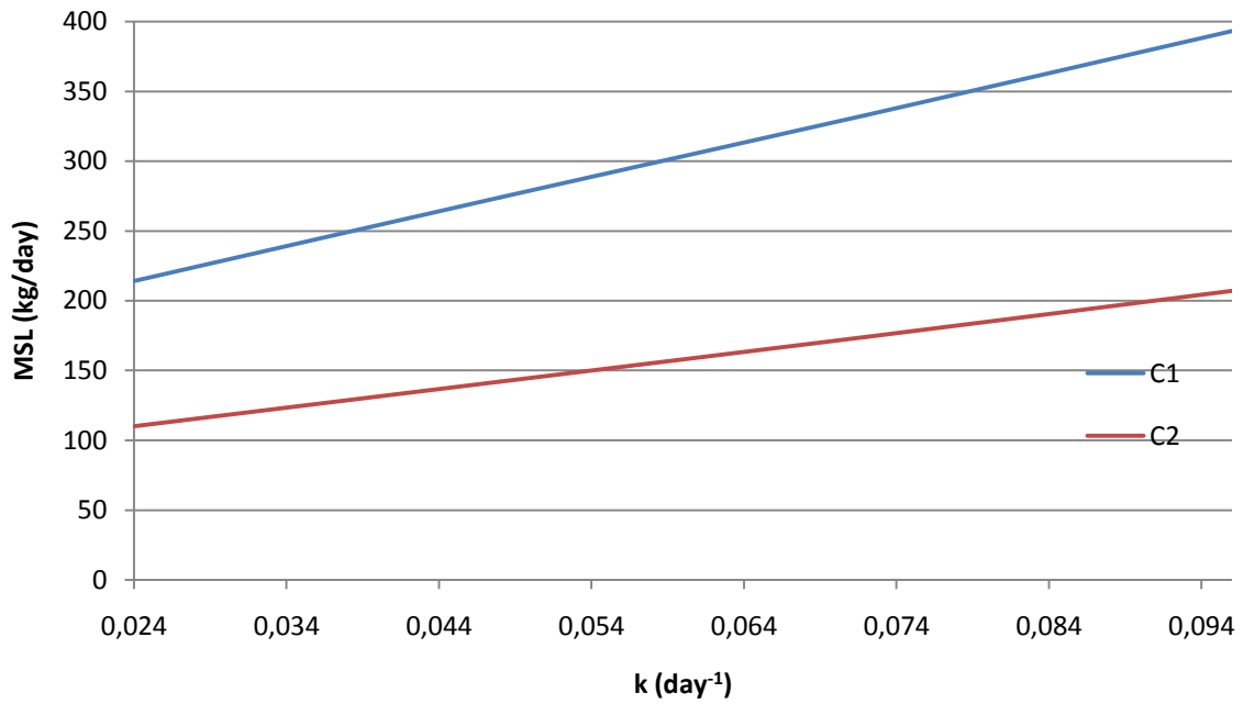
Figure 44: MSL related to variability in removal rates
