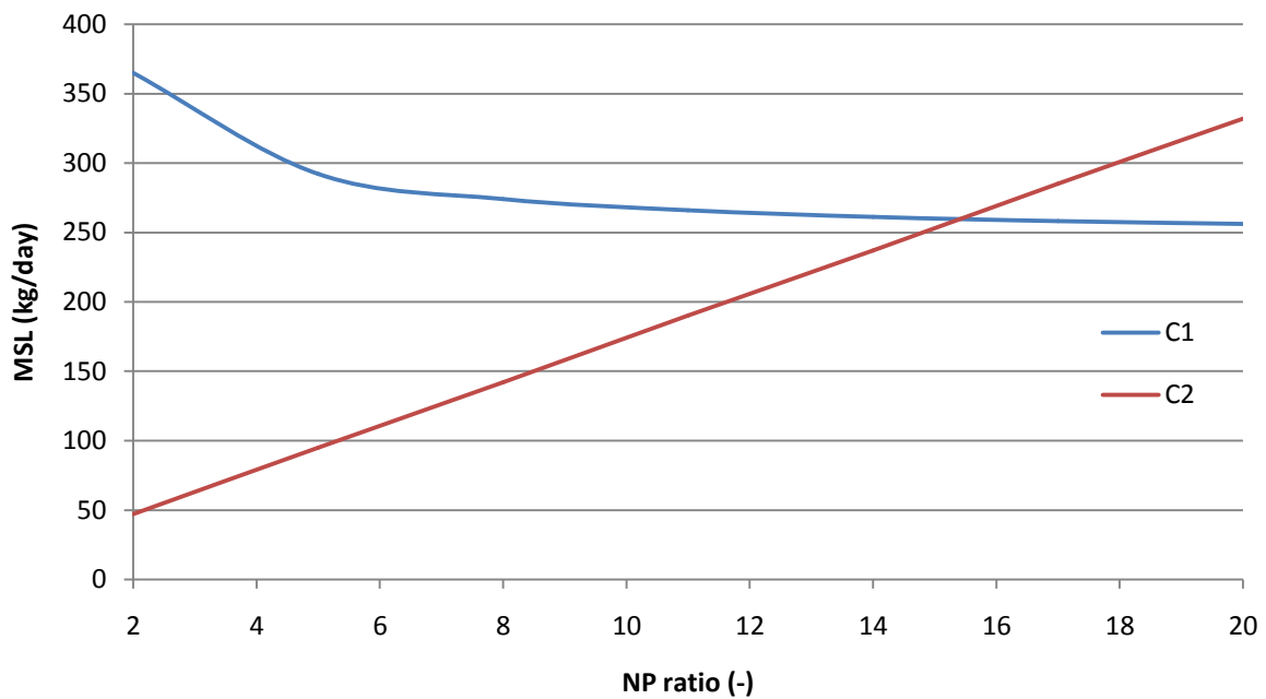
Figure 45: MSL related to variability in the nitrogen and phosphorus ratio of the load
