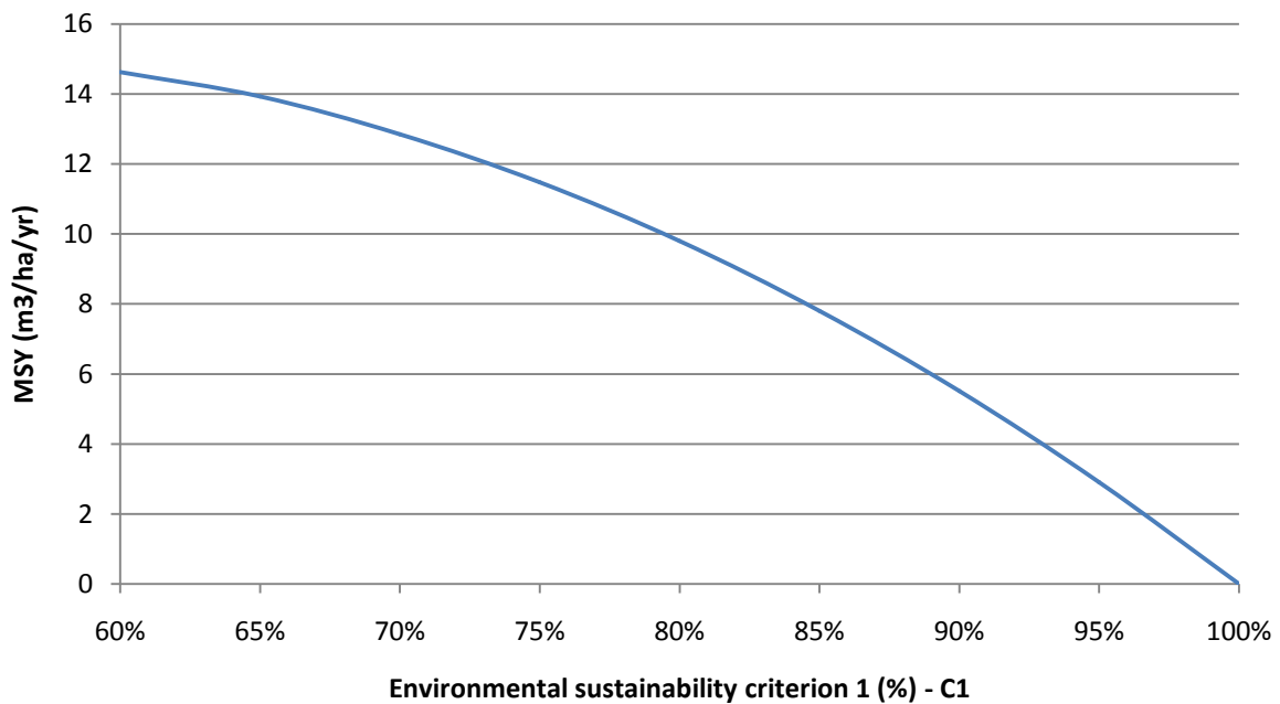
Figure 30: MSY related to variability of C1
