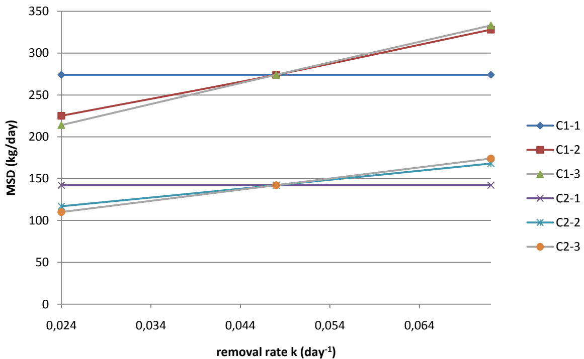
Figure 62: Influence of different types of criteria on the MSL for changing pollutant removal rates
