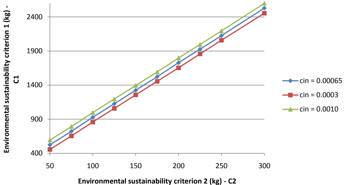
Figure 55: Relation between C1 and C2 for varying background concentrations
