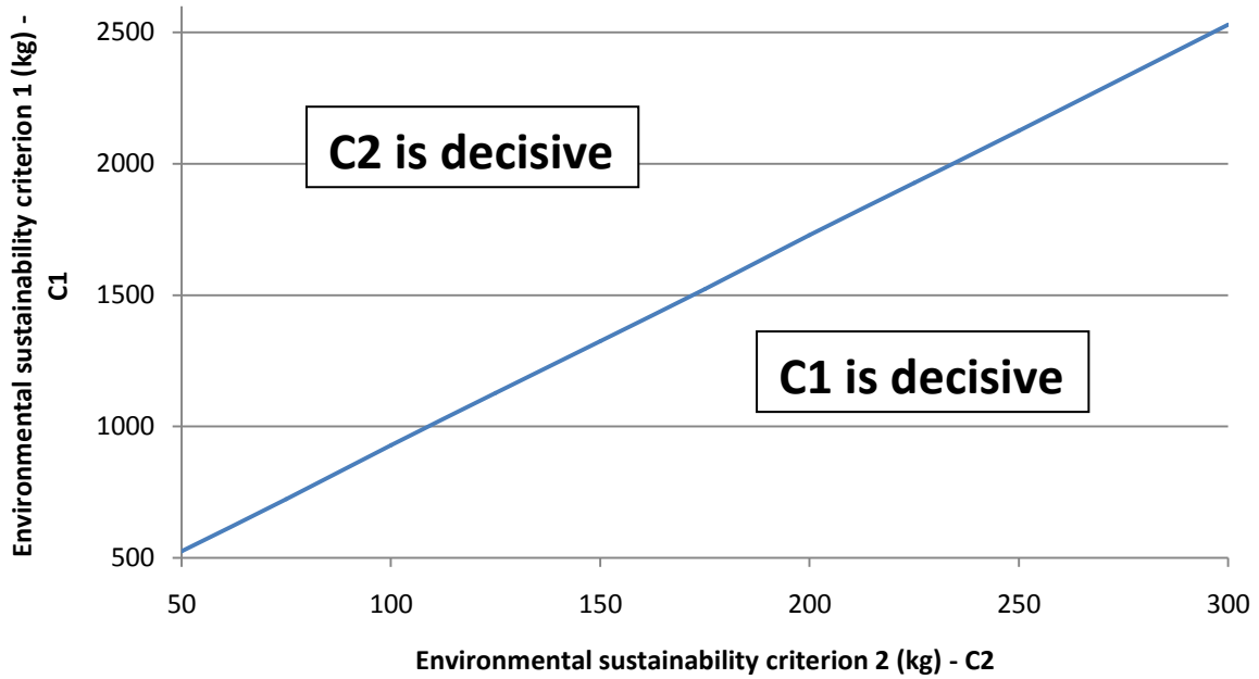
Figure 51: Relation between C1 and C2 for pollution in a lake
