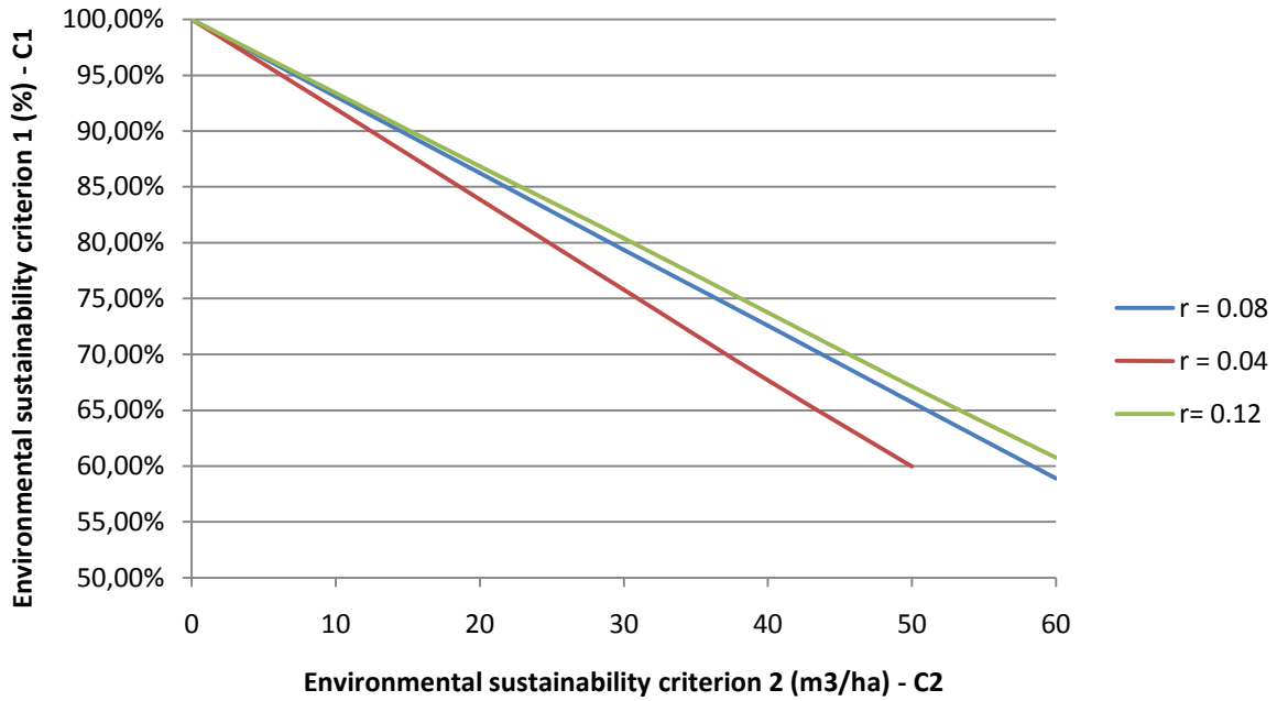
Figure 35: Relation between C1 and C2 for varying grow rates
