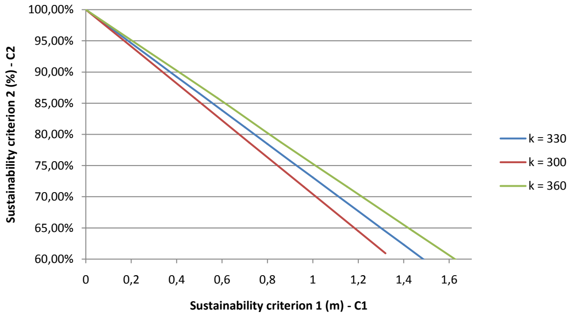
Figure 20: Relation between C1 and C2 for varying values of the residence time
