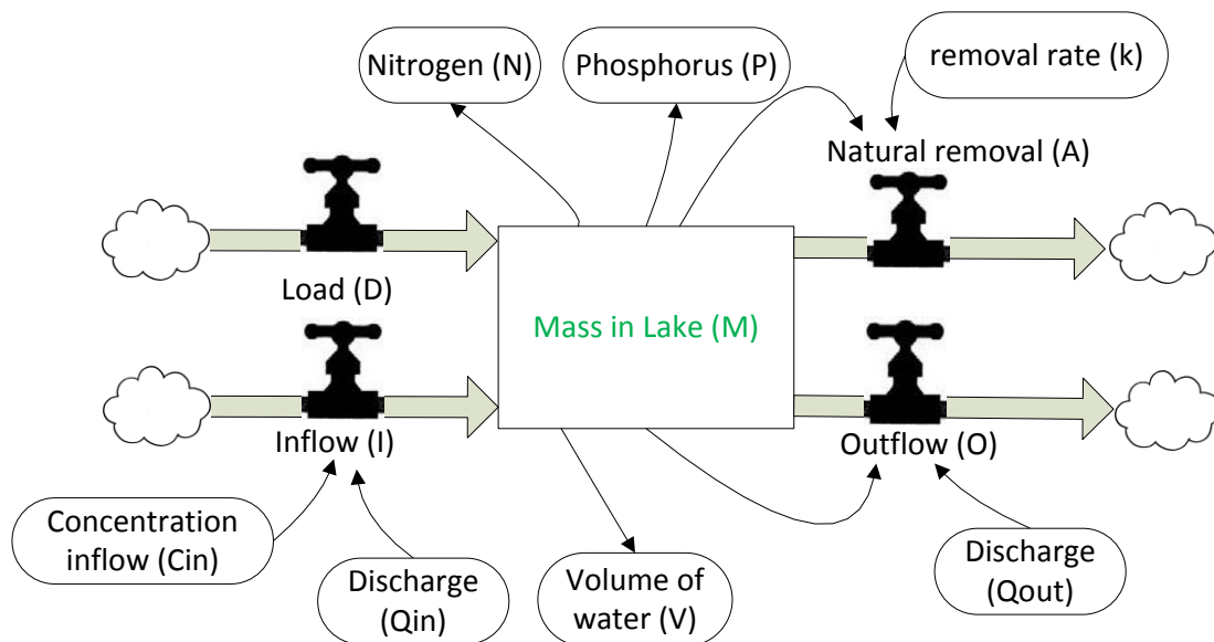
Figure 39: Flow stock diagram of pollution in a lake
