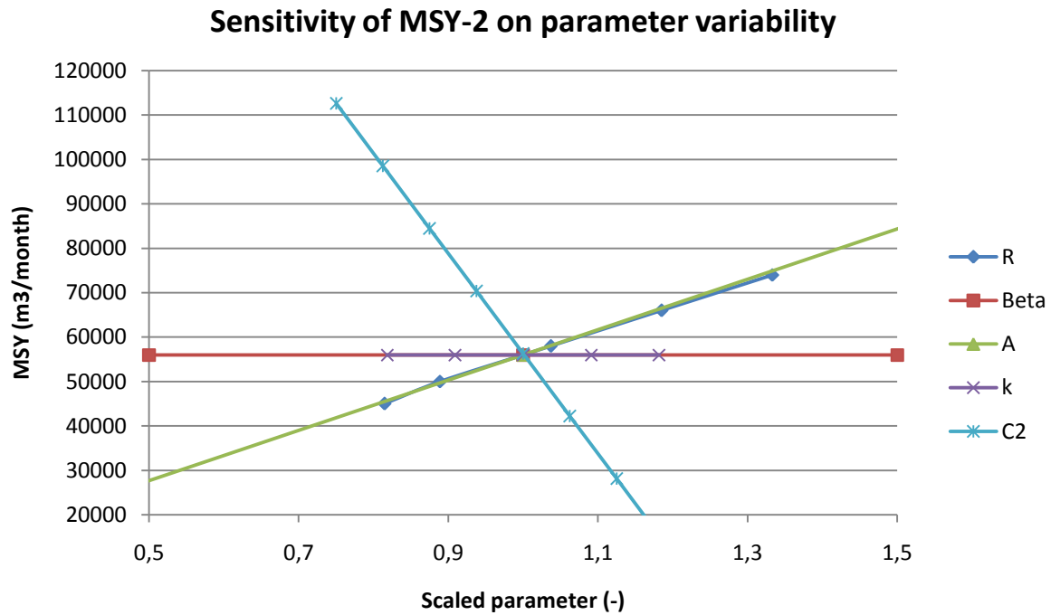
Figure 15: Sensitivity of MSY on parameter variability for C2
