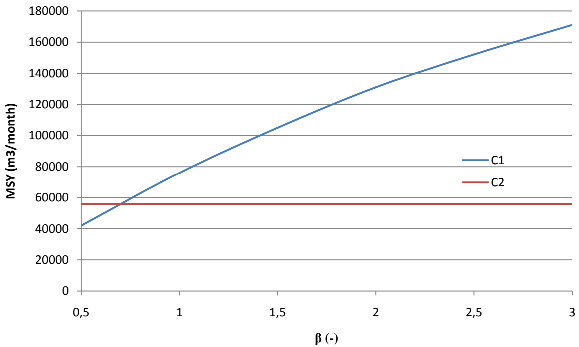
Figure 9: MSY related to variability of beta
