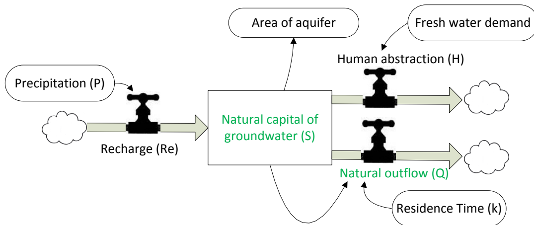
Figure 3: System diagram of a groundwater model
