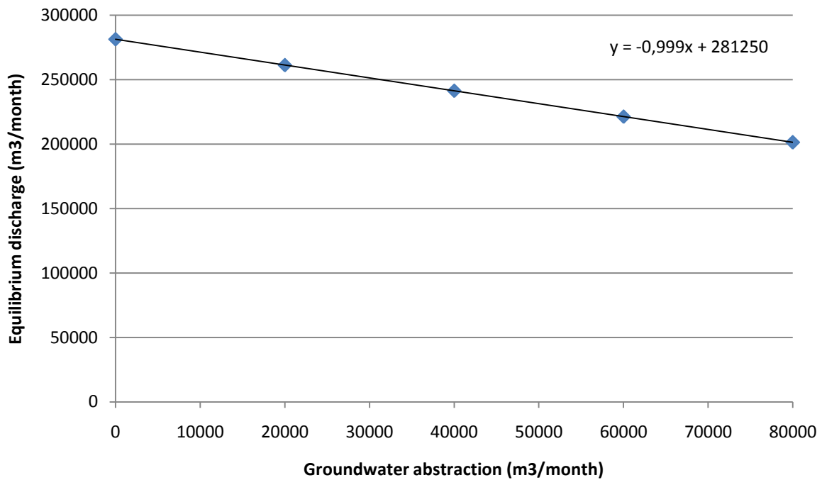
Figure 7: Relation between groundwater abstraction rates and equilibrium groundwater discharge
