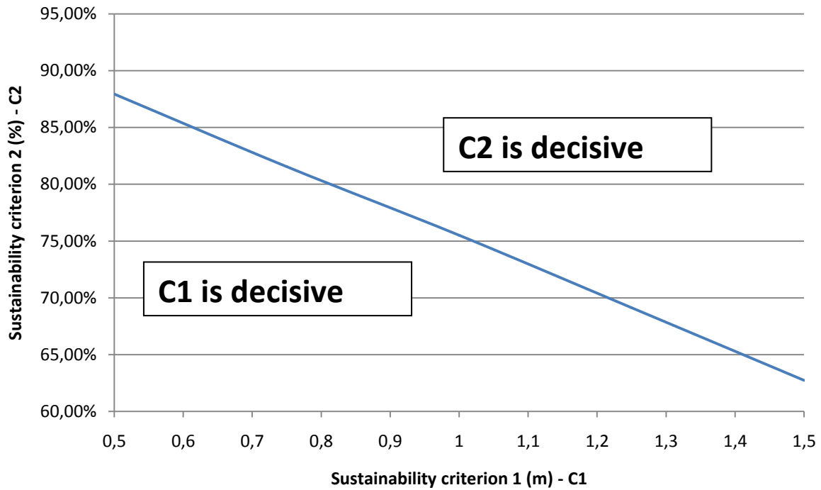
Figure 16: Relation between C1 and C2 for groundwater
