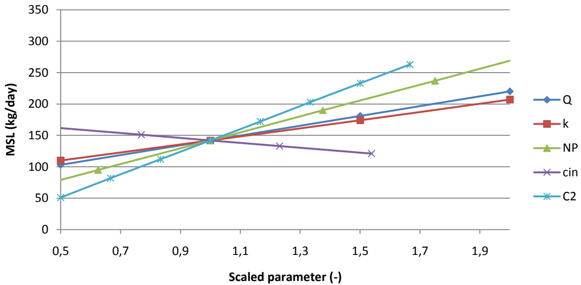
Figure 50: Sensitivity of MSL on parameter variability for C2
