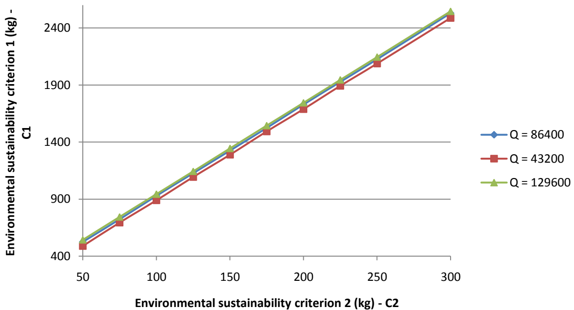
Figure 52: Relation between C1 and C2 for varying discharge values
