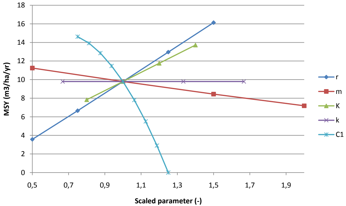
Figure 32: Sensitivity of MSY on parameter variability for C1
