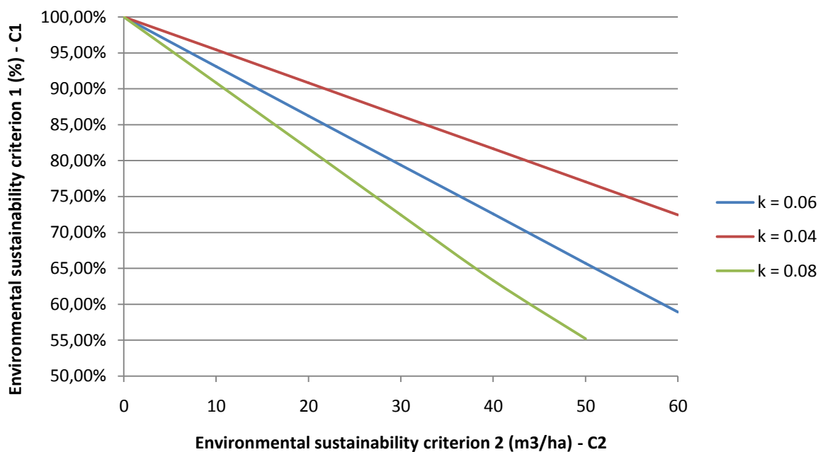
Figure 38: Relation between C1 and C2 for varying decomposition rates
