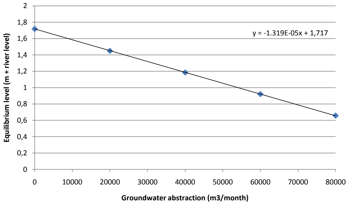
Figure 6: Relation between groundwater abstraction and equilibrium groundwater level
