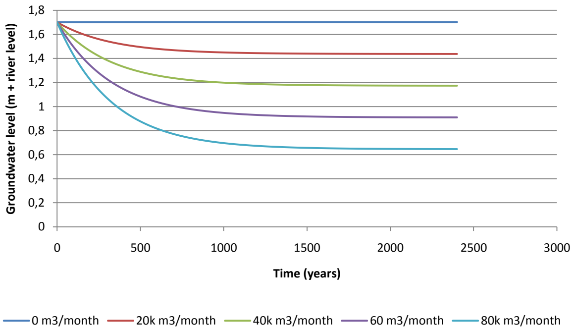
Figure 5: Groundwater levels over time with different abstraction rates
